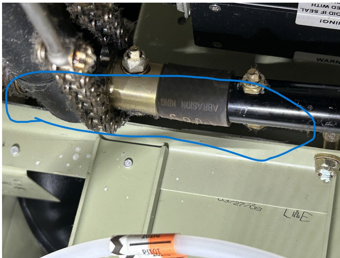
Photograph 6 - Closeup View of Bending of Elevator Control Pivot Point (Courtesy of FAA)
