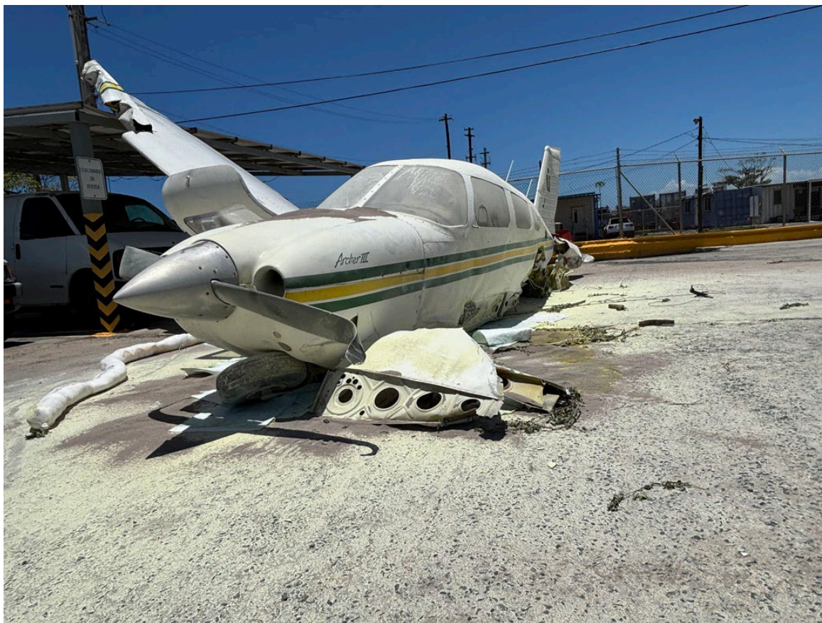
Photograph 1 - Main Wreckage (Courtesy of FAA)
