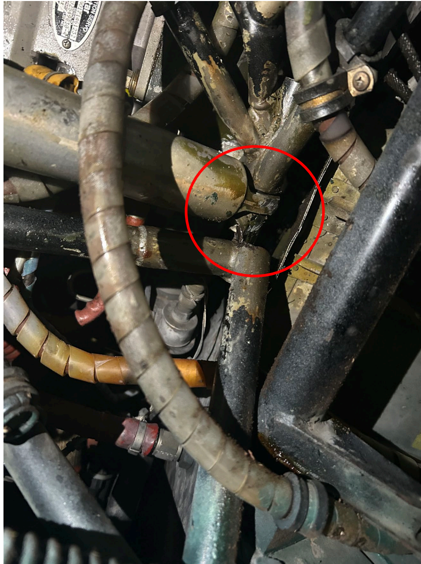
Photograph 3 - Broken Engine Mount Beside Nose Gear Retract Cylinder (Courtesy of Mechanic)
