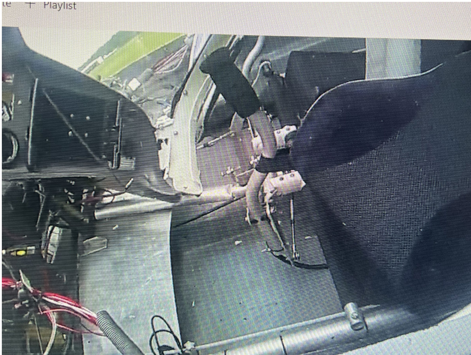
Photograph 3 - View of the seat cushion strap around control stick. (Courtesy of VCSO)
