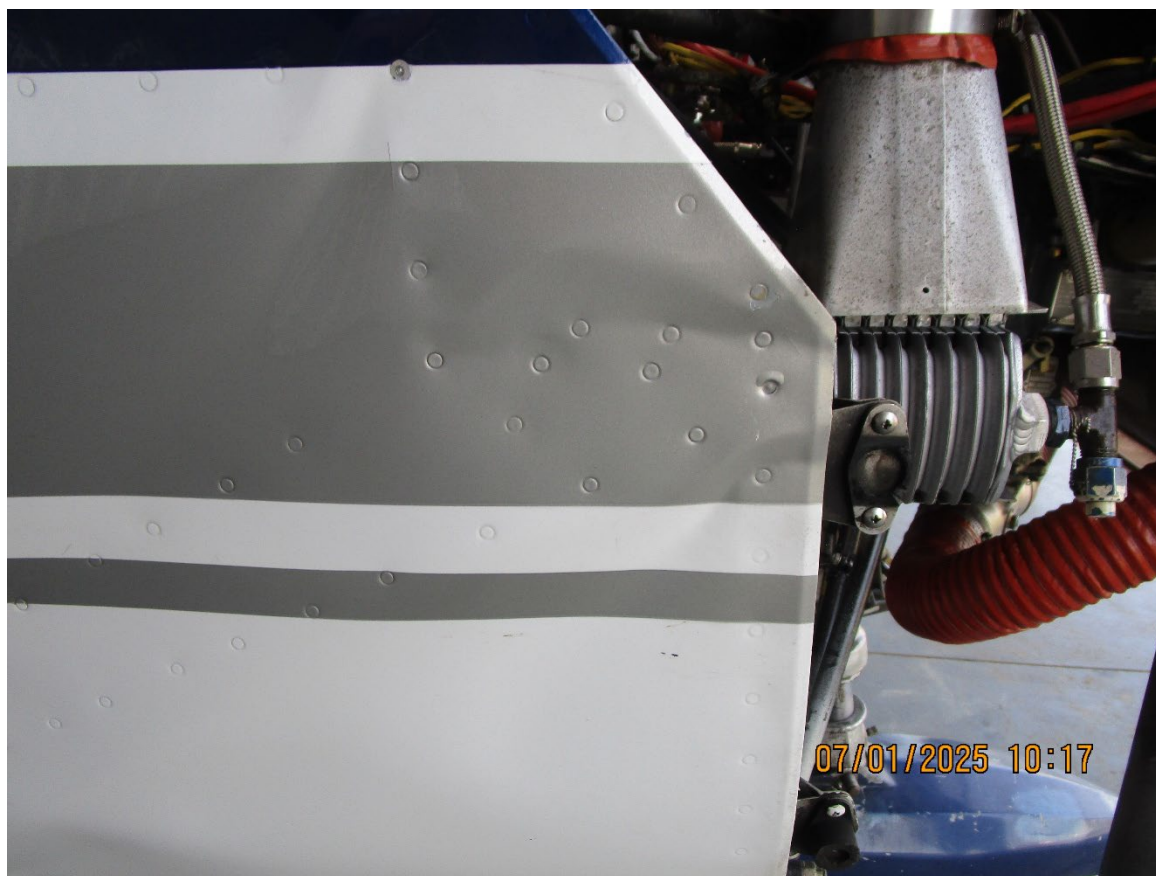
Photograph 4 - Close up of damage to right side of fuselage (Courtesy of FAA)
