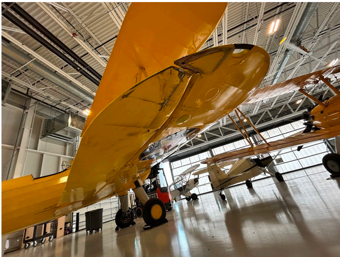
Photograph 2 - Exterior Damage to Lower Right Wing (Courtesy of FAA)
