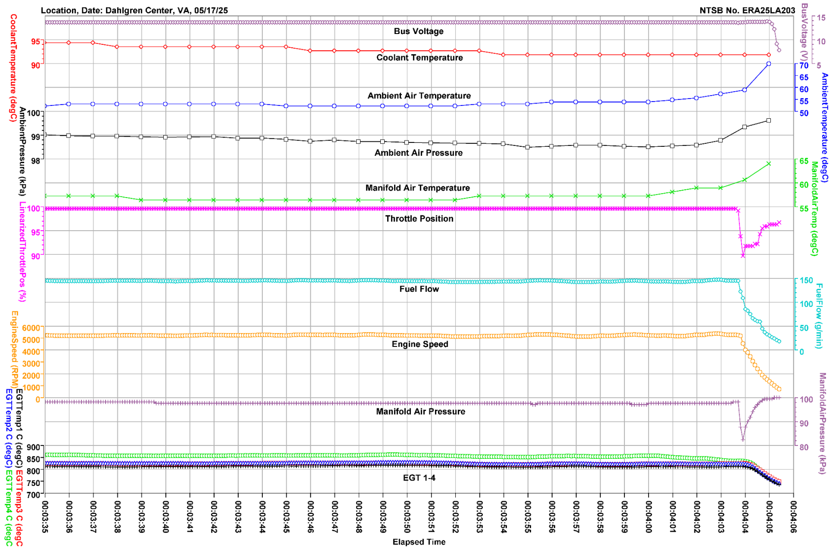
Plot of LaneA parameters for approximately the final 30 seconds of recorded data.
