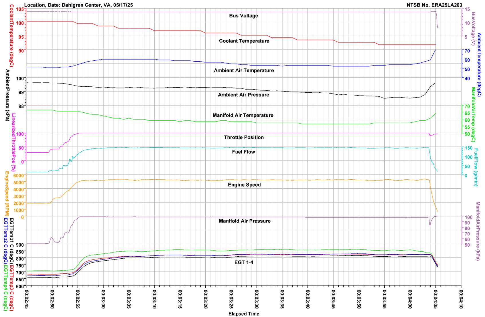
Plot of LaneA parameters for the accident event.
