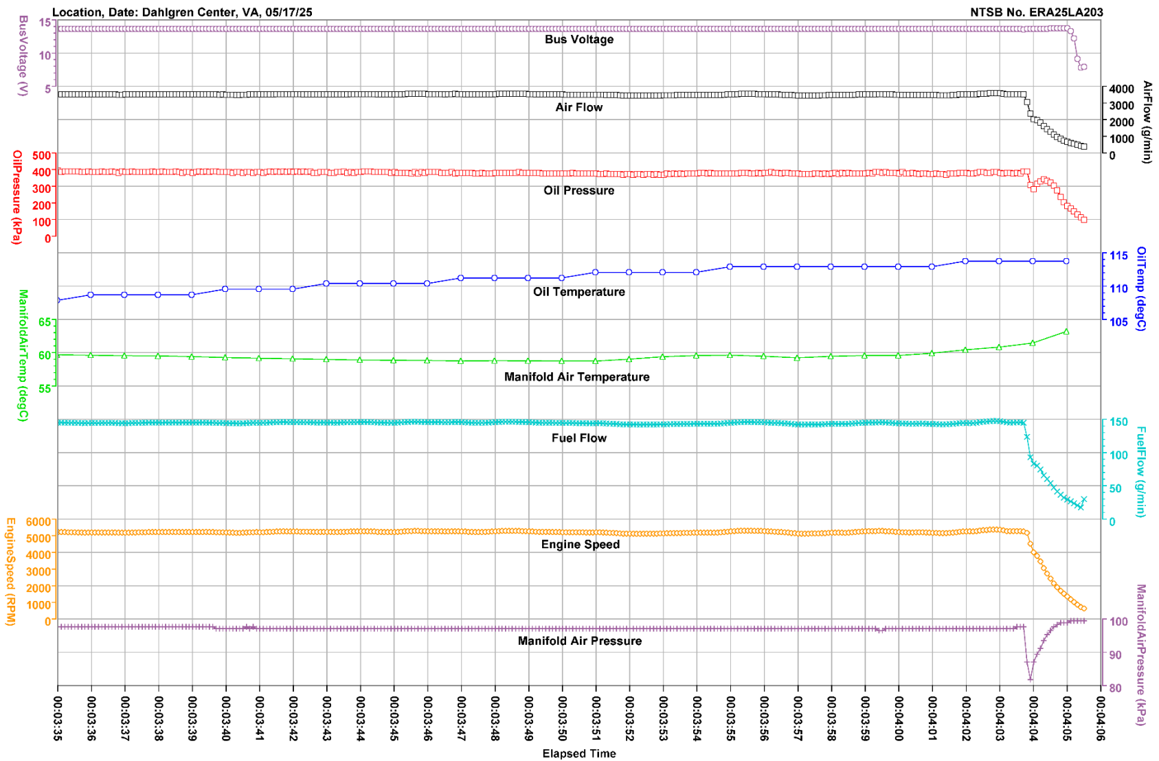
Plot of LaneB parameters for approximately the final 30 seconds of recorded data.
