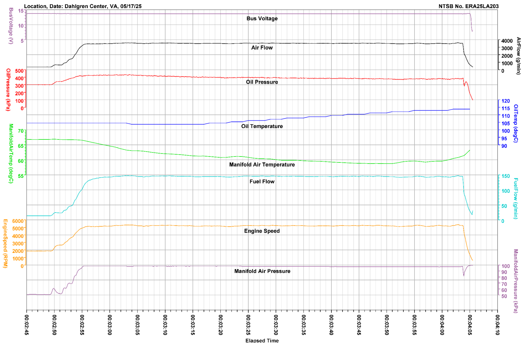
Plot of LaneB parameters for the accident event.
