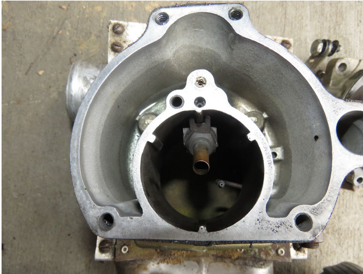
Photograph 7 - Carburetor Bowl (Courtesy of Lycoming)
