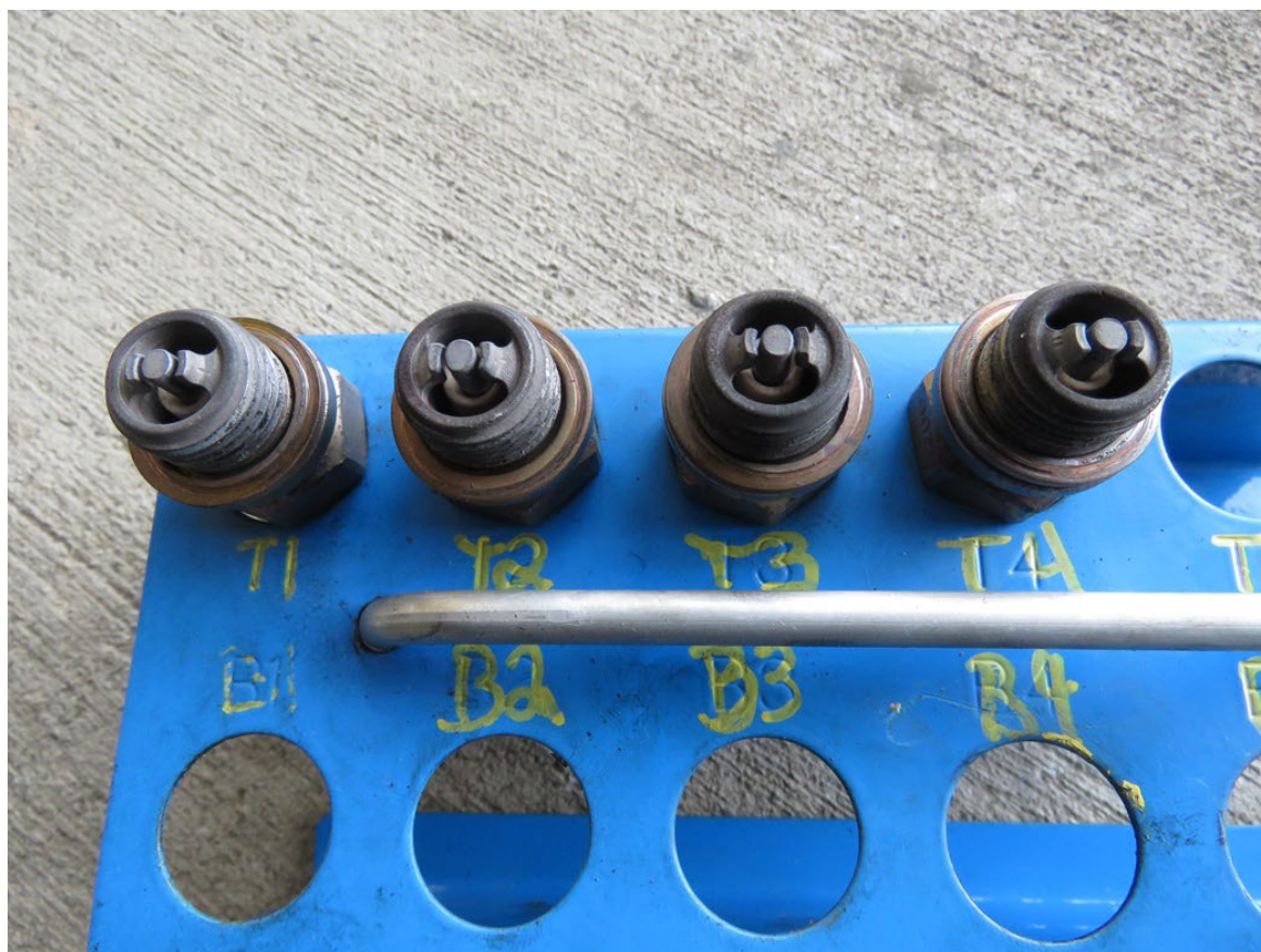
Photograph 5 - Top Spark Plugs (Courtesy of Lycoming)
