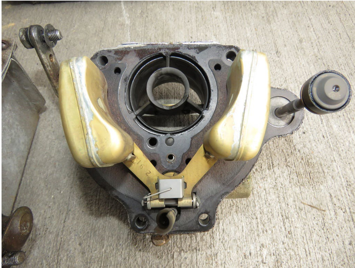
Photograph 8 - Carburetor Floats (Courtesy of Lycoming)
