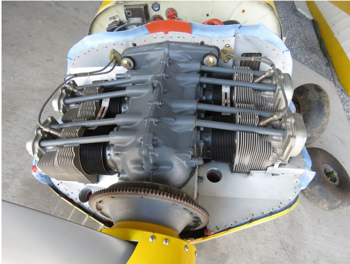
Photograph 4 - Engine (Courtesy of Lycoming)
