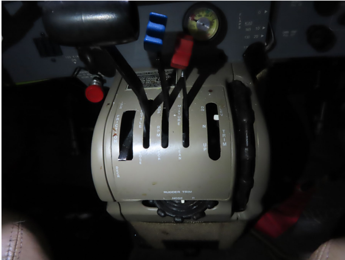
Photograph 6 - Throttle Quadrant and Flap Handle (Courtesy of Piper Aircraft)
