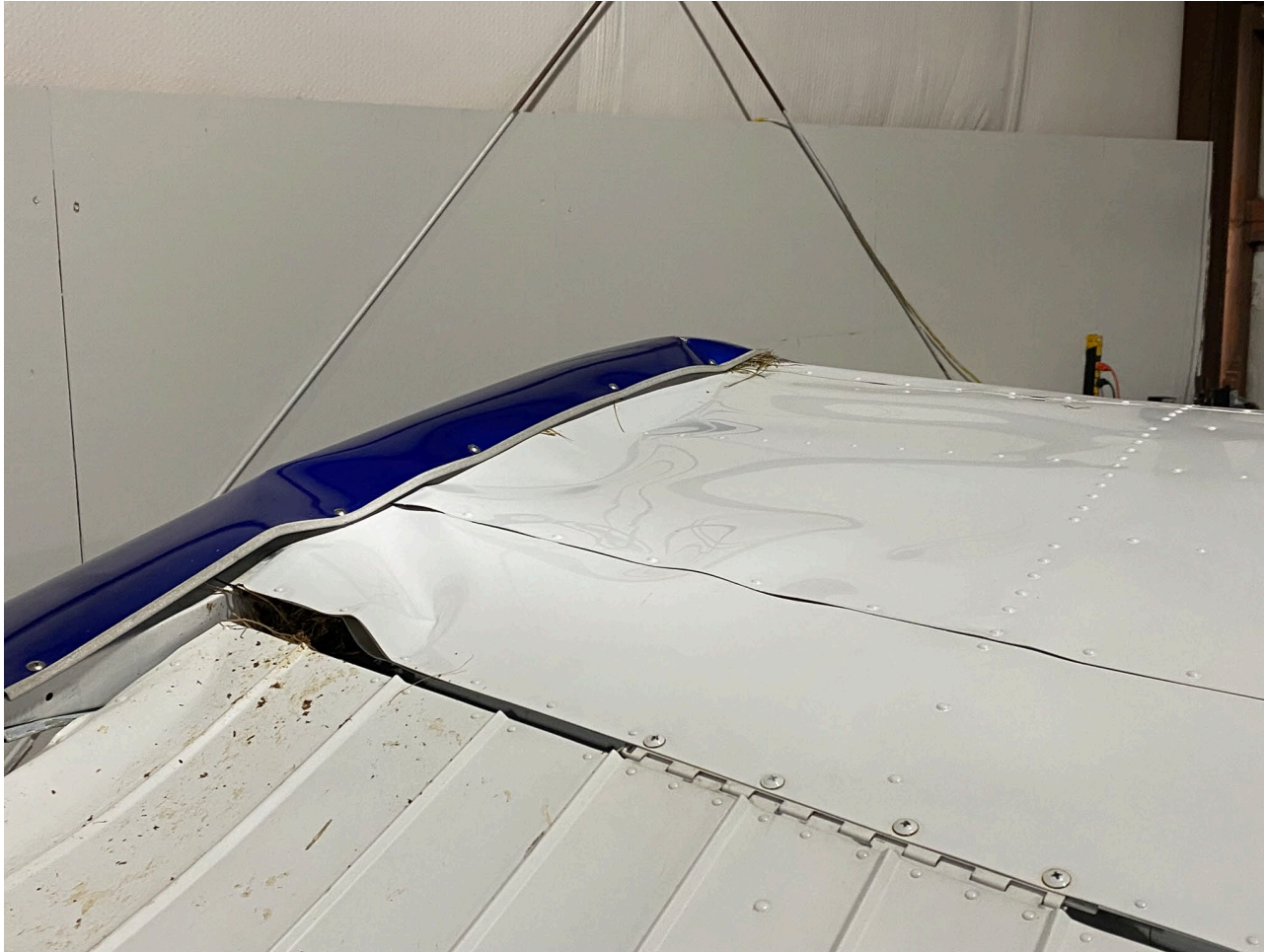
Photograph 3 - View of top of left wing damage. (Courtesy of FAA)
