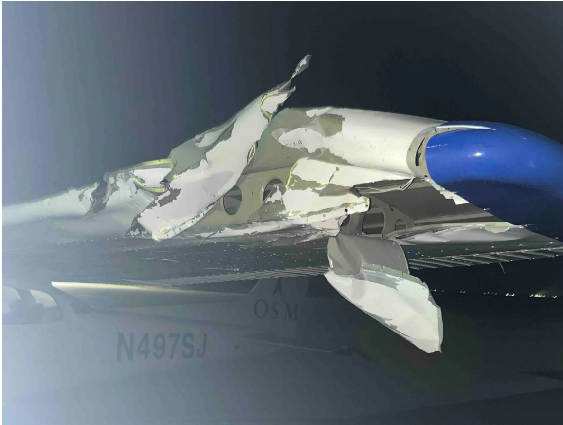
Photograph 2 - Cessna Left Wing (Courtesy of FAA)
