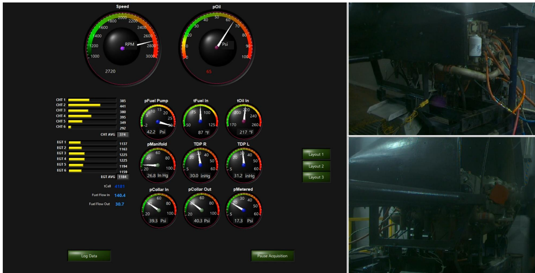
Photograph 1 - Screenshot of engine run video (at full throttle) with engine data (Source: CAT)
