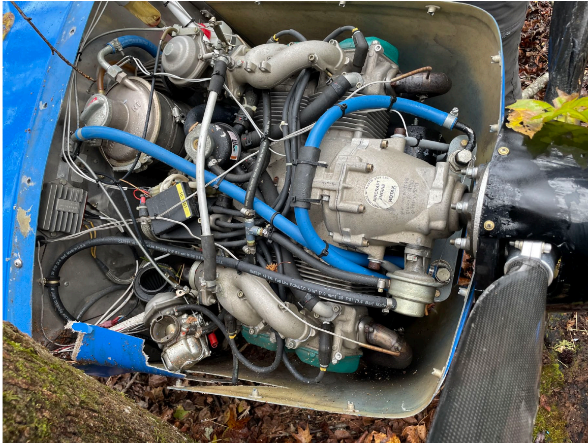
Photograph 3 - Engine and Propeller Hub (Courtesy of FAA)
