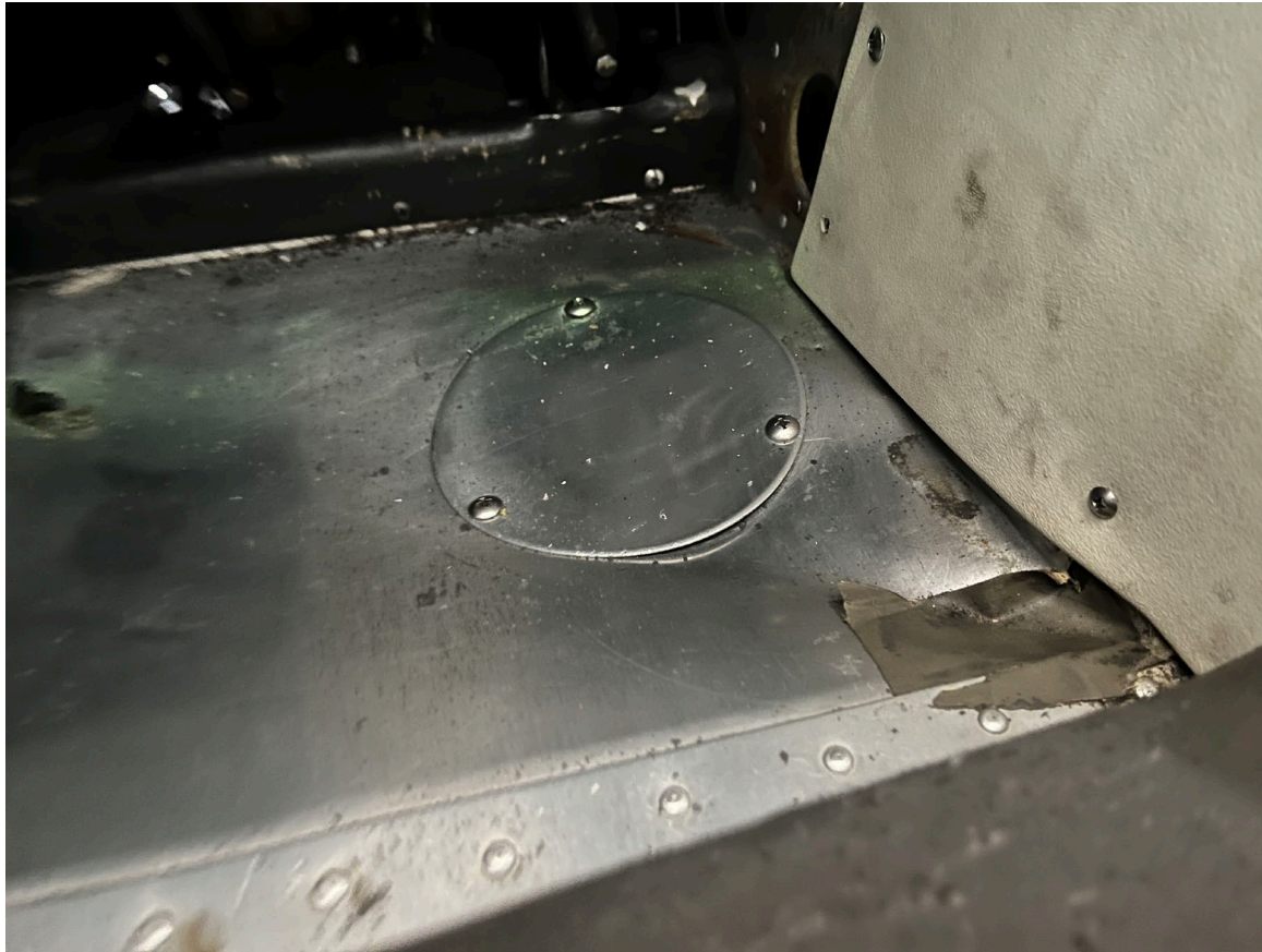
Photograph 3 - Floorboard wrinkling (Courtesy of FAA)
