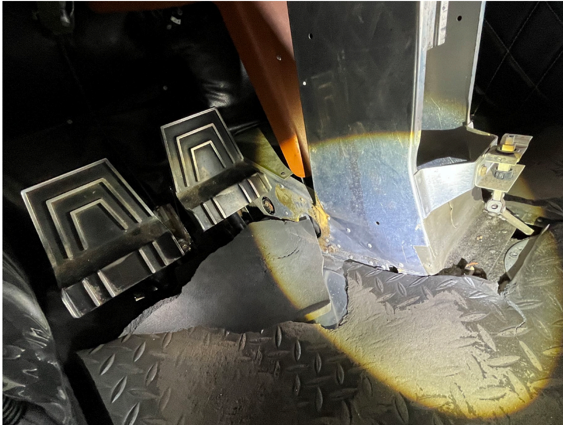
Photograph 2 - Structure wrinkling (Courtesy of FAA)
