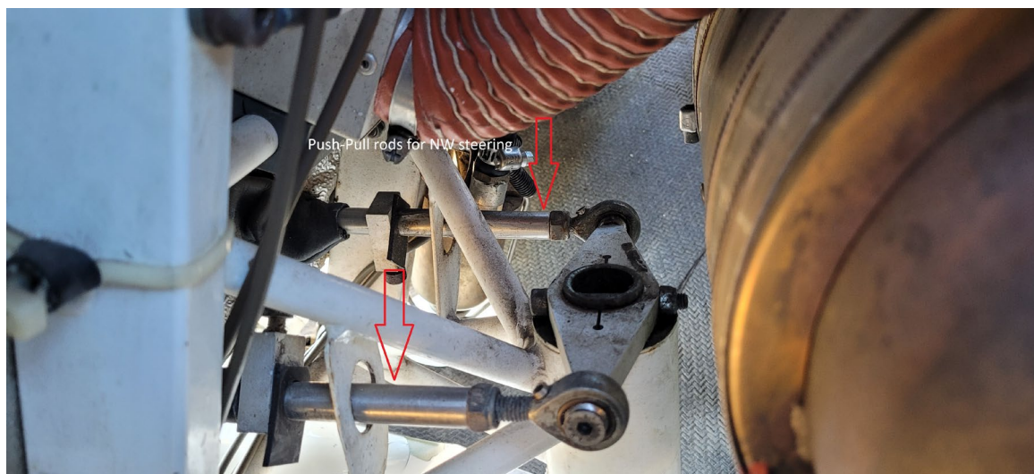
Photograph 5 - Nosewheel Steering Linkage (Courtesy of FAA)
