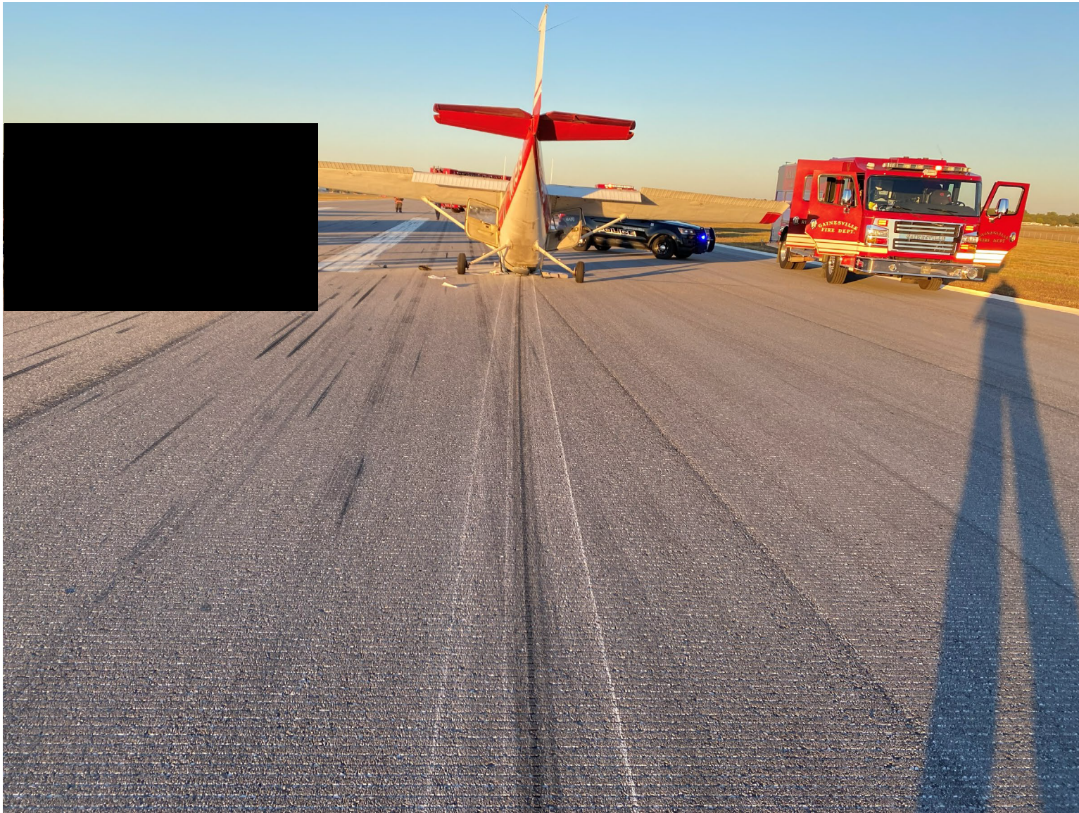
Photograph 2 - N11519 on Runway 05 at Lee Gilmer Memorial Airport (Courtesy of Gainesville PD)
