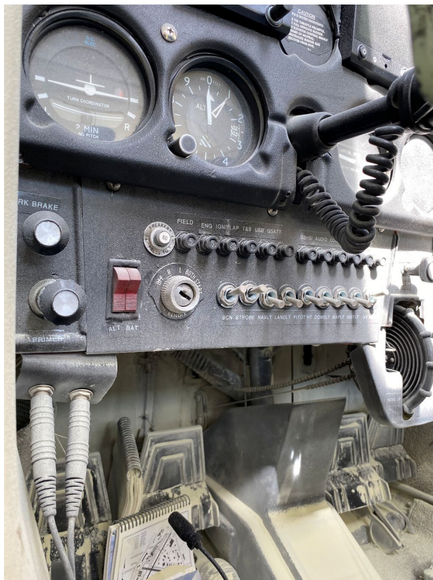
Photograph 4 - Cockpit Floor Area with Residue from Discharged Fire Extinguisher (Courtesy of FAA)
