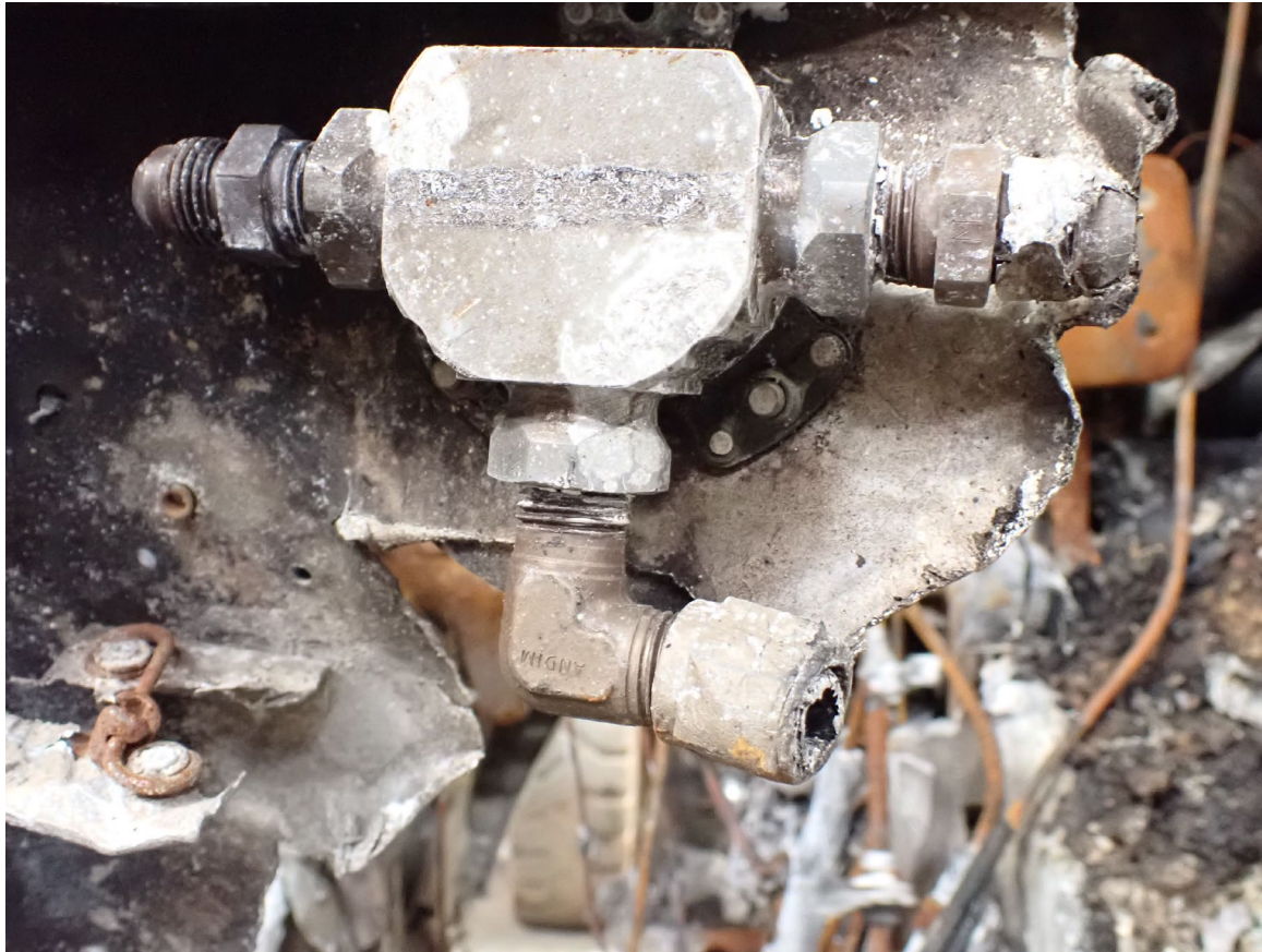
Photograph 4 - Thermal damage noted to the fuel selector valve (NTSB)
