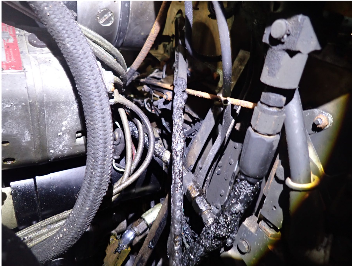
Photograph 6 - Thermal damage noted to hydraulic lines (NTSB)
