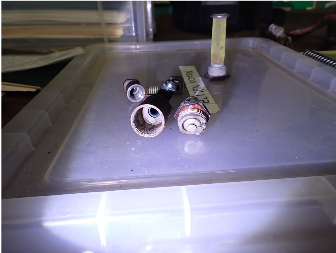
Photograph 5 - Fuel pressure regulator and check valve (NTSB)
