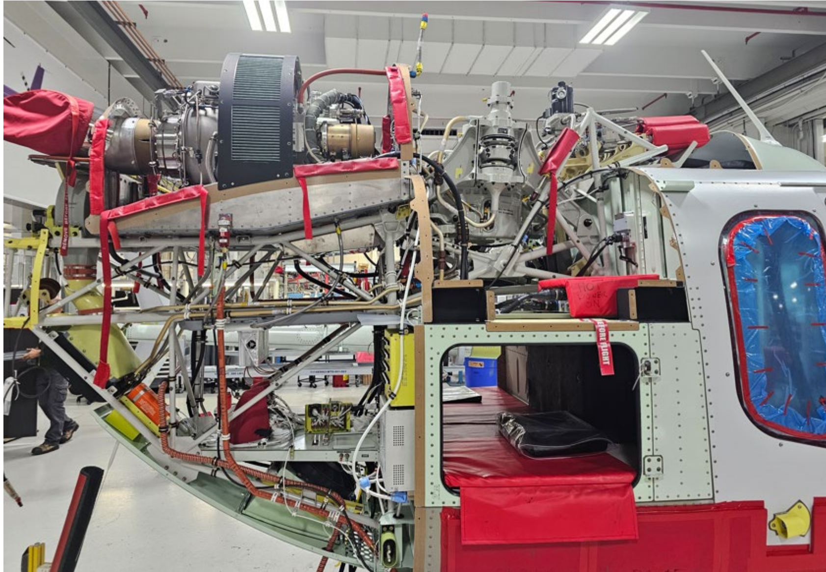
Side view pictures showing the truss on an aircraft on the assembly line
