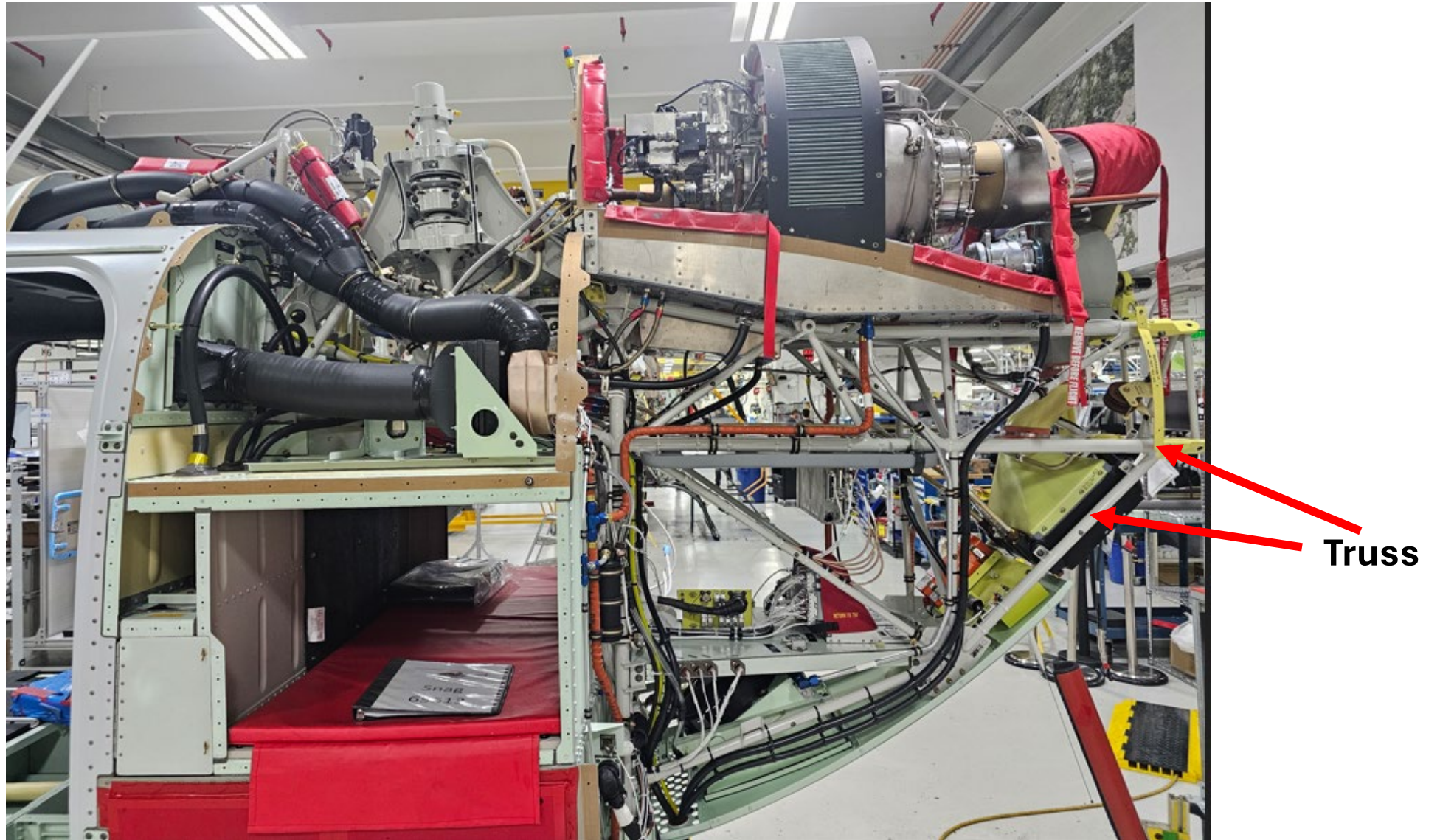
Side view showing the truss on an aircraft on the assembly line
