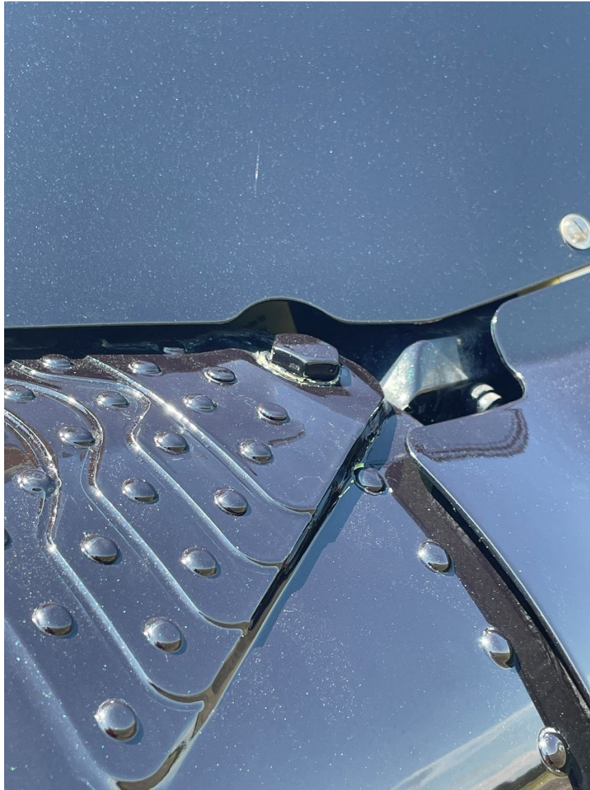
Photograph 2 - Damage to tail cone assembly (Source: Operator)
