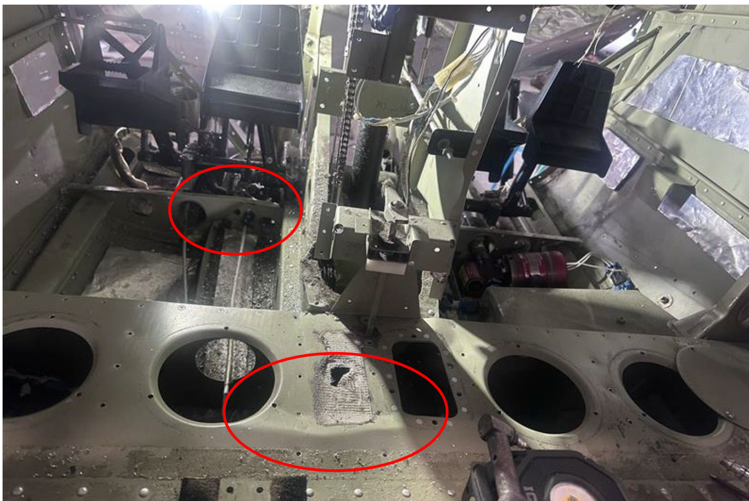
Photograph 2 - Internal structure impact damage (Courtesy of Flight School)
