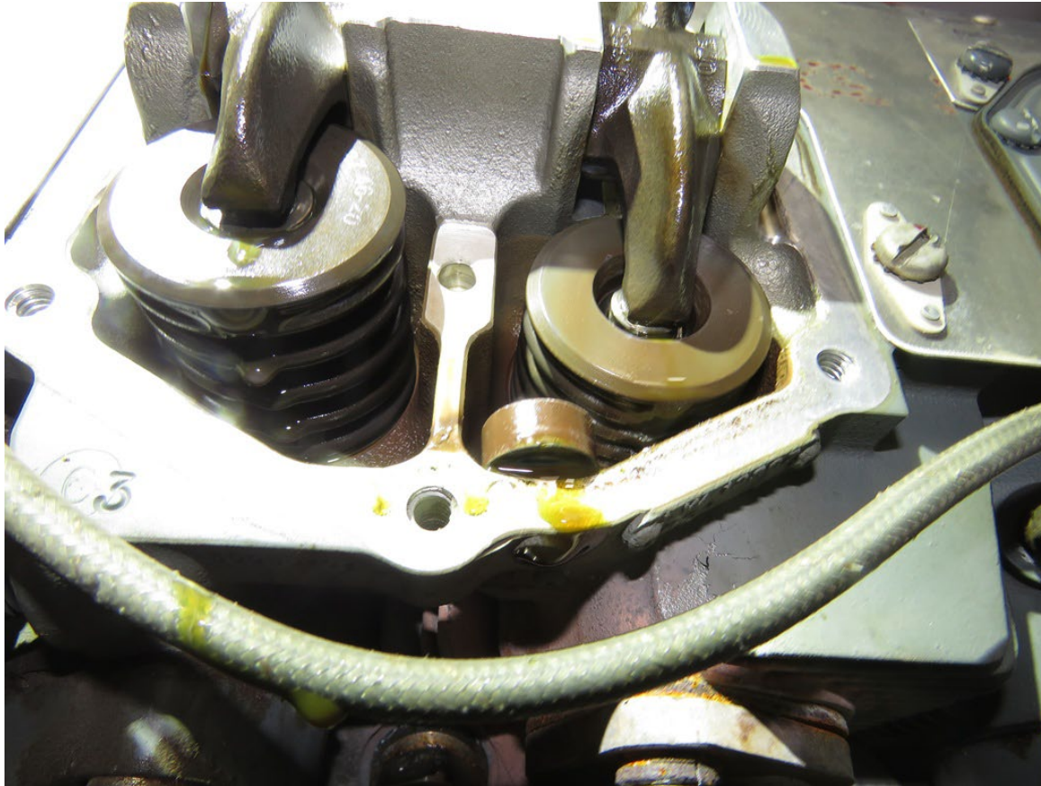
Photograph 7 - No. 3 Cylinder at Engine Exam (Courtesy of Lycoming)
