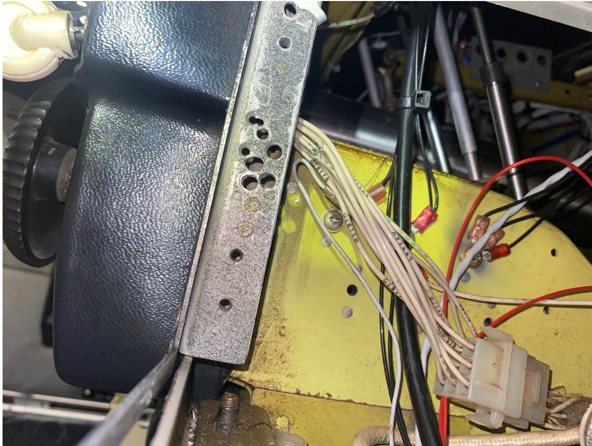
Photograph 1 - Landing gear switch wiring (Courtesy of FAA)
