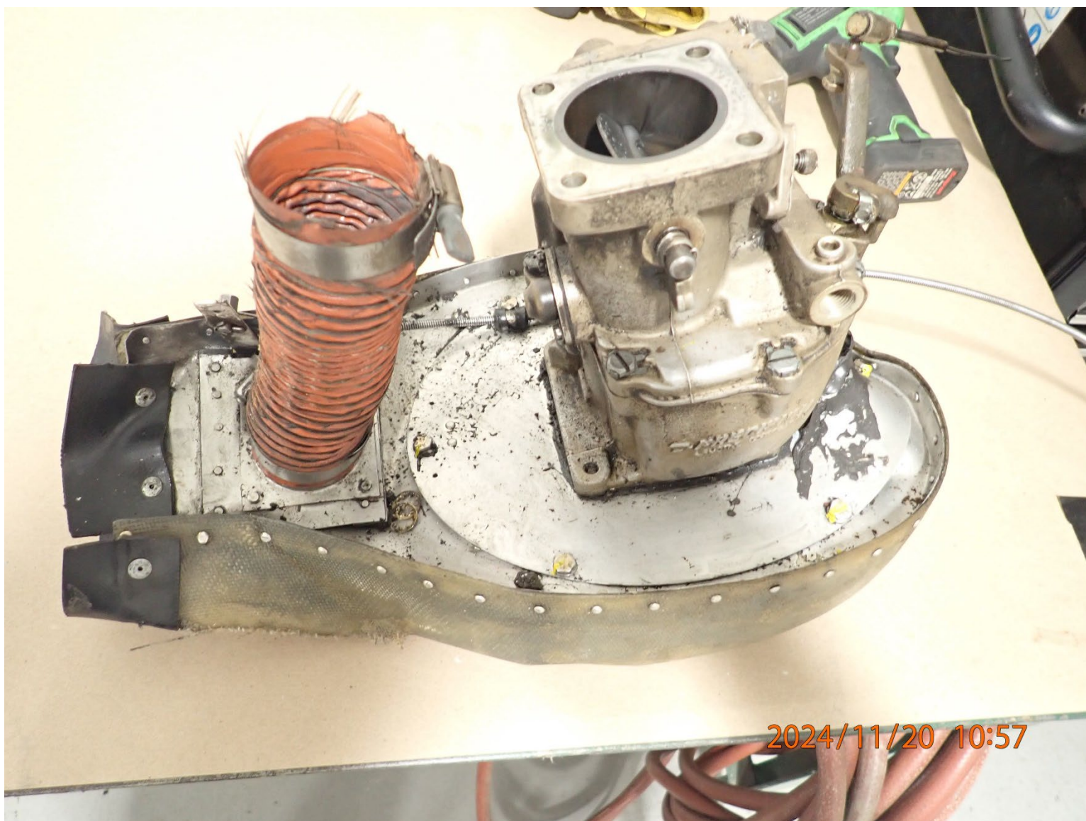
Photograph 5 - Carburetor and airbox
