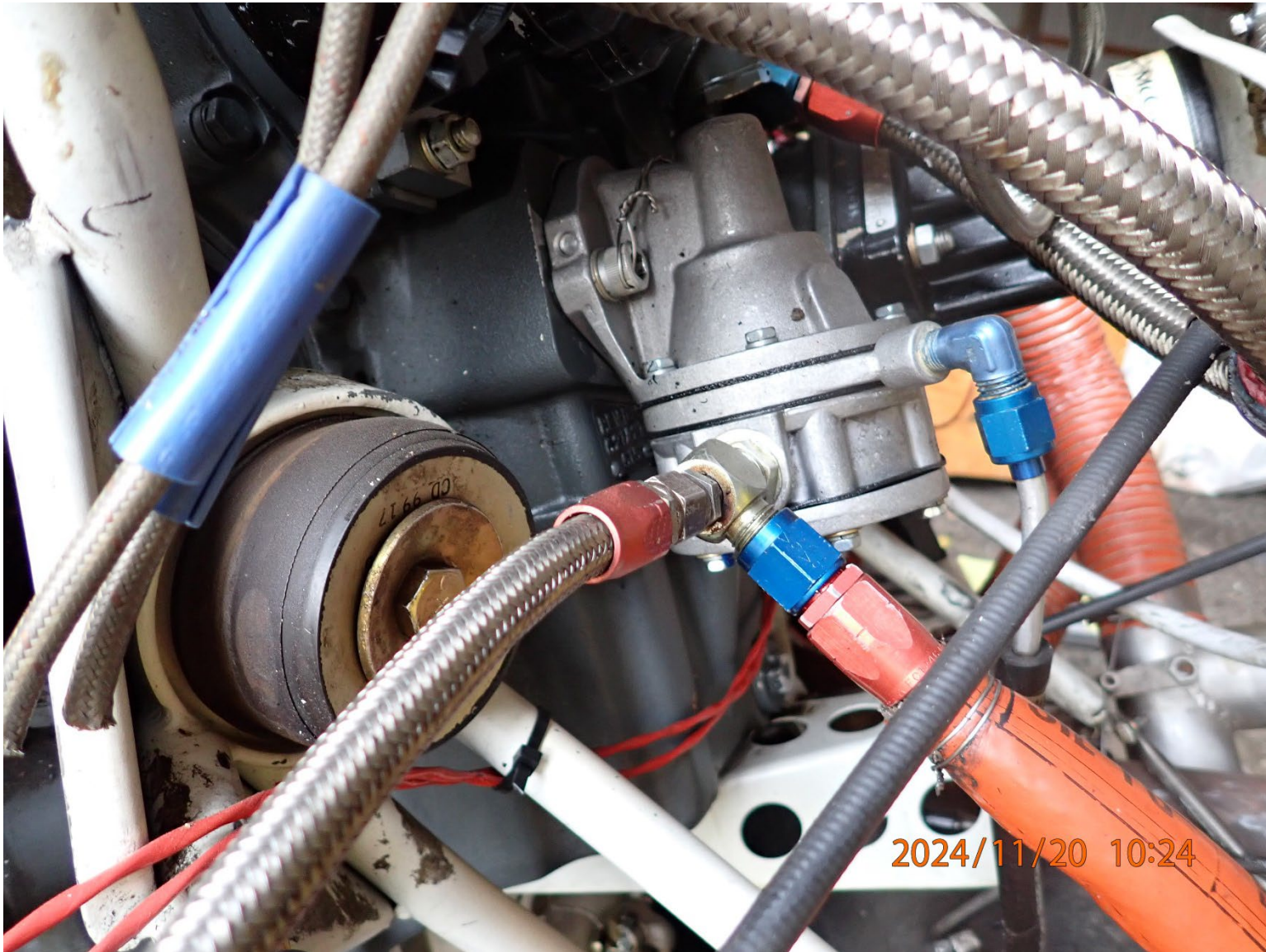
Photograph 4 - Diaphragm fuel pump and fuel lines
