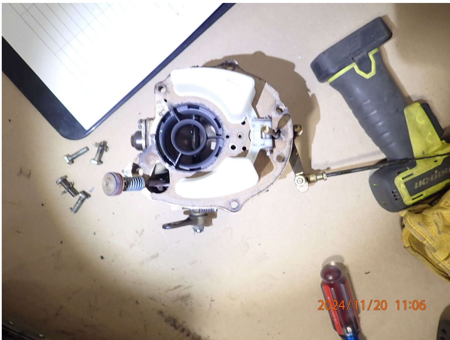
Photograph 7 - Carburetor floats, mixture control, and accelerator pump
