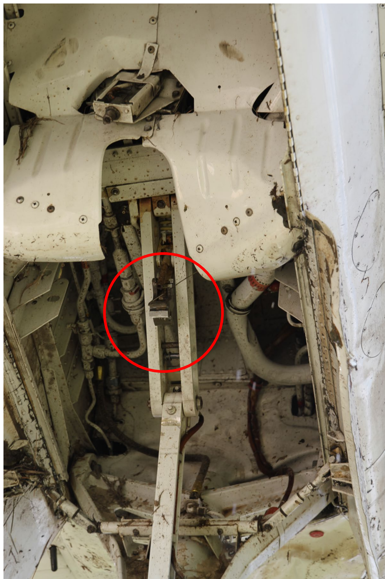
Photograph 4 - Broken Left Main Actuator Clevis (Courtesy of FAA)
