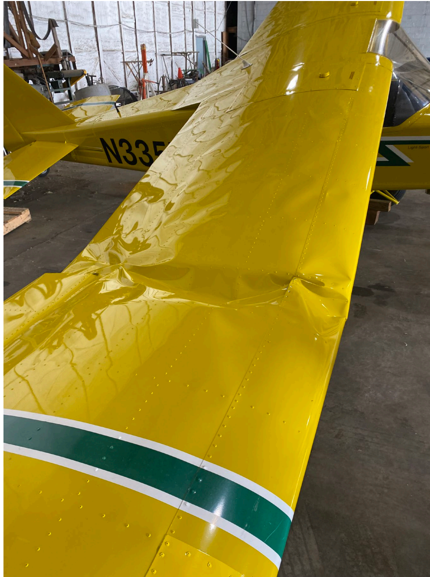
Photograph 2 - Right wing impact damage (Courtesy of FAA)
