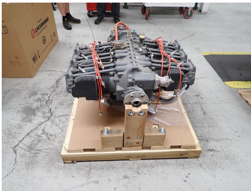
Photograph 4 - Engine front (Courtesy of Lycoming)
