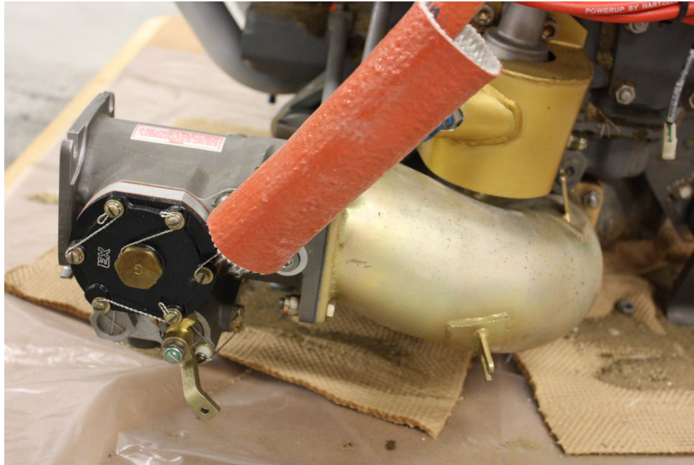
Photograph 6 - Fuel servo mounted to intake horn (Courtesy of NTSB)
