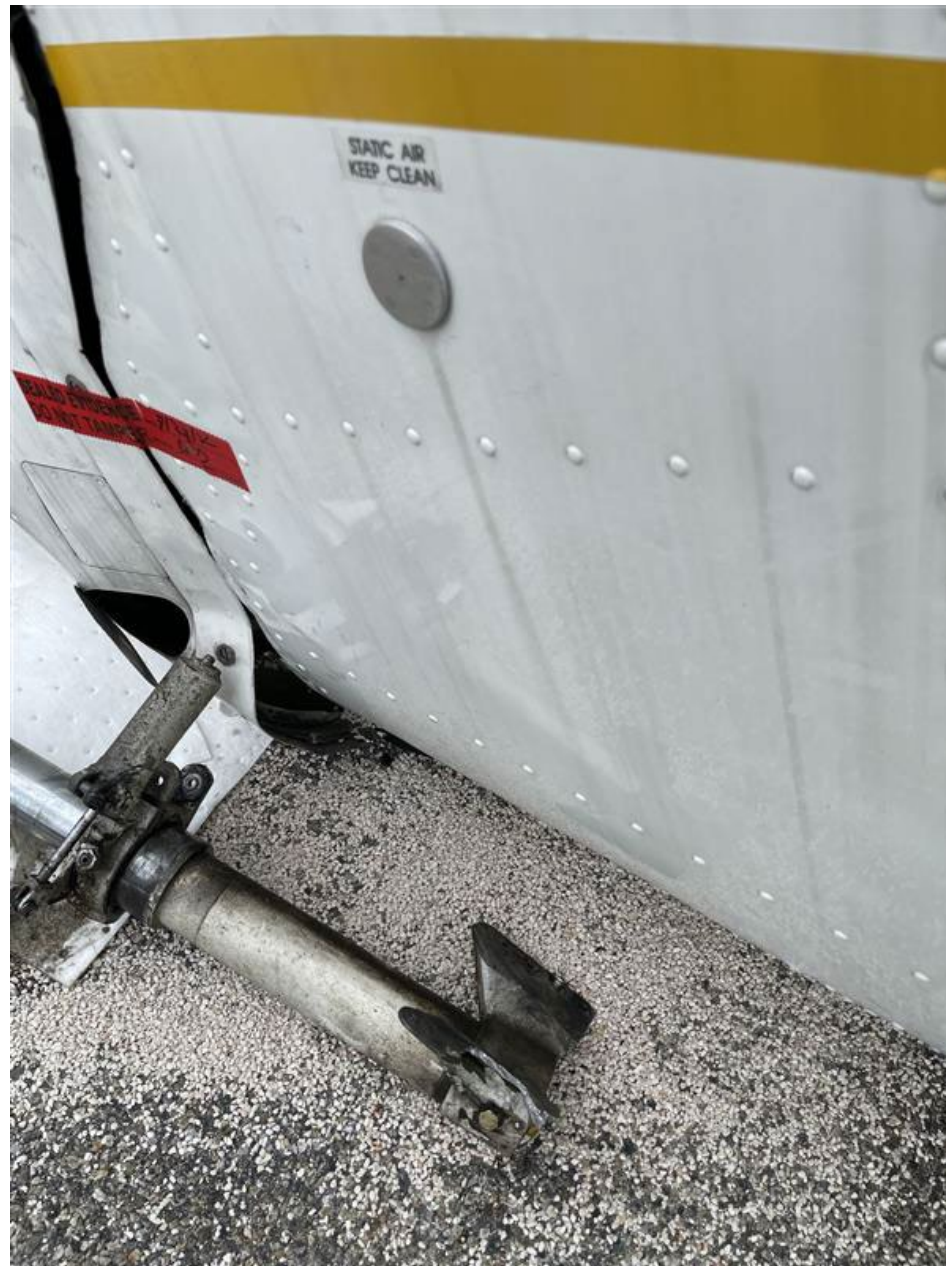
Photo 4 – View of Fractured Nose Landing Gear (N/L/G) Mount Structure Attached to Separated N/L/G (FAA)
