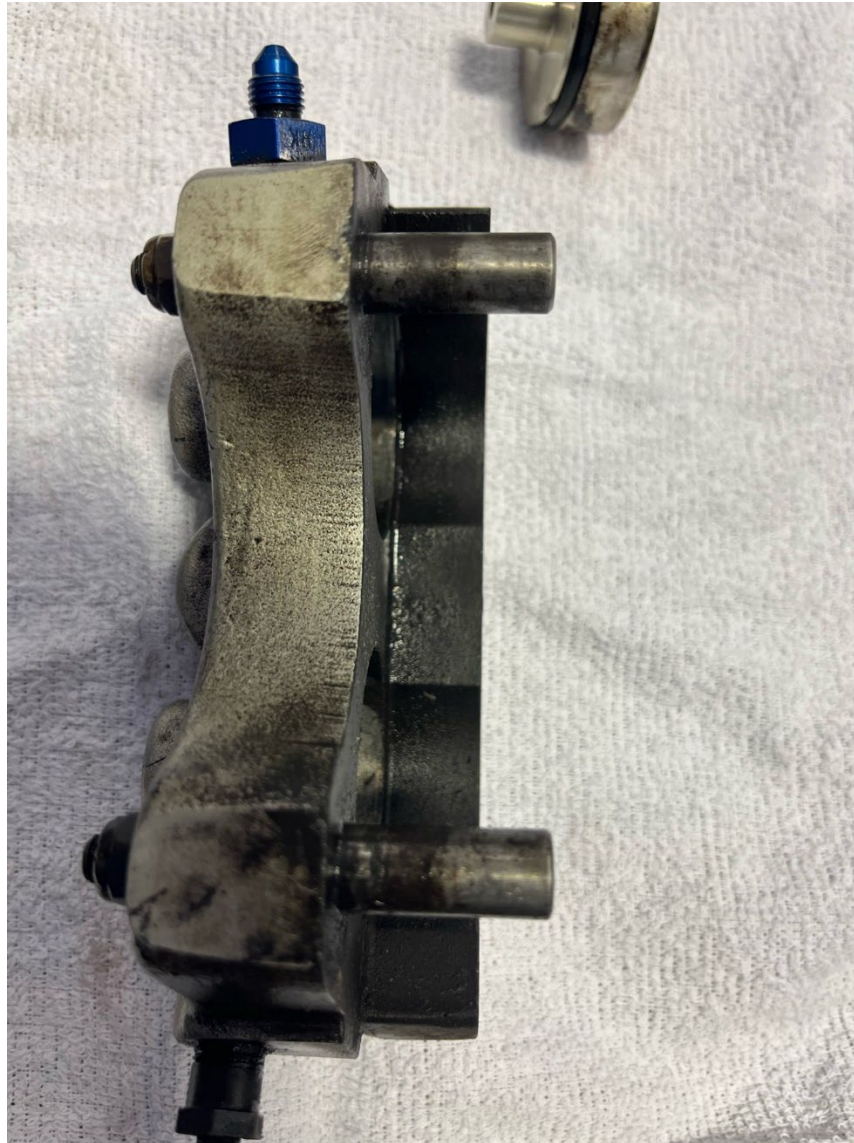
Photograph 7 - Disassembled right brake caliper (Courtesy of mechanic)
