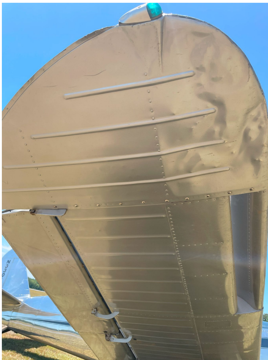
Photograph 3 - Right Wingtip Postaccident (Courtesy of FAA)
