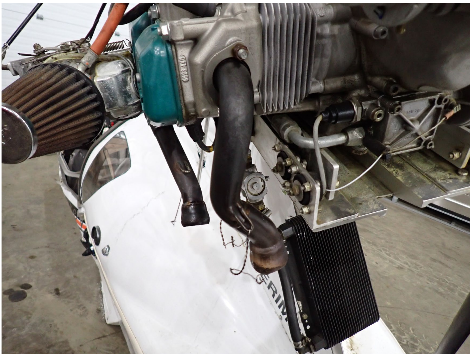
Photograph 6 - No. 1 exhaust riser
