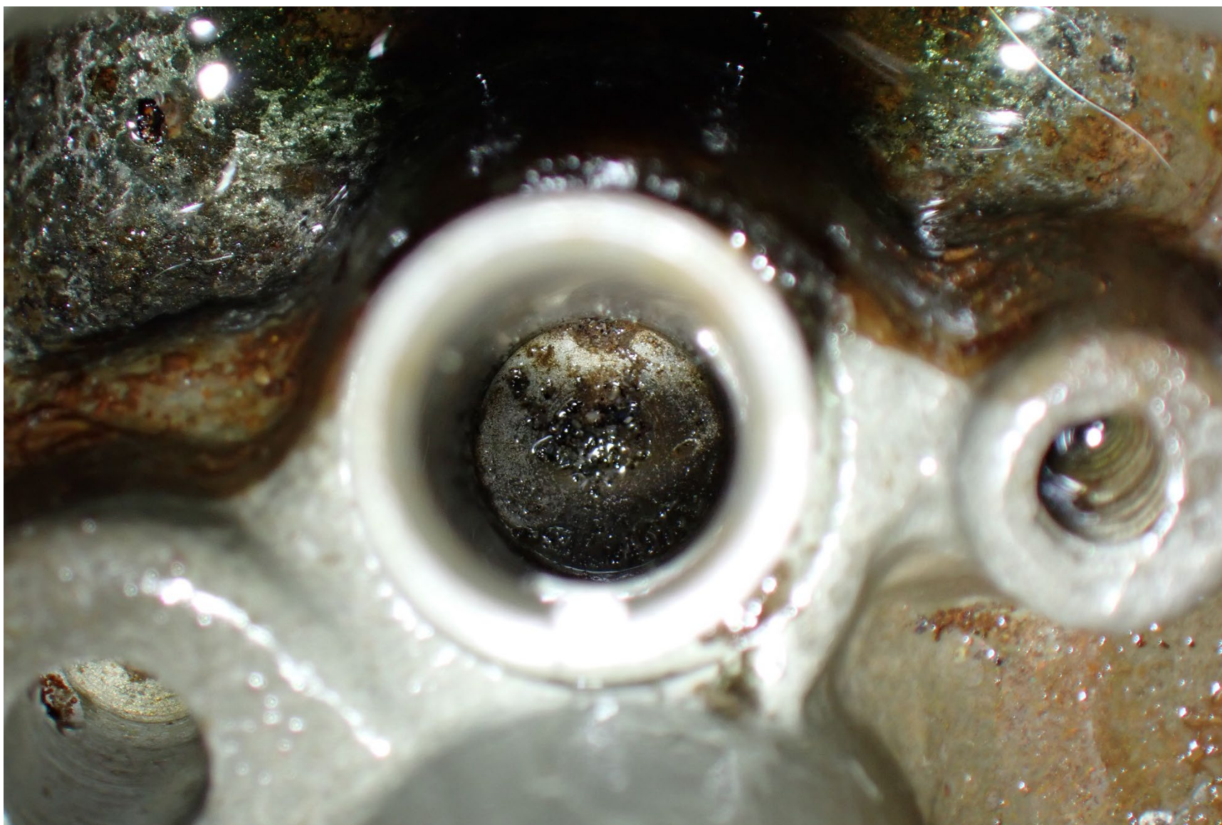
Photograph 11 - Debris found in carburetor mixture control sleeve
