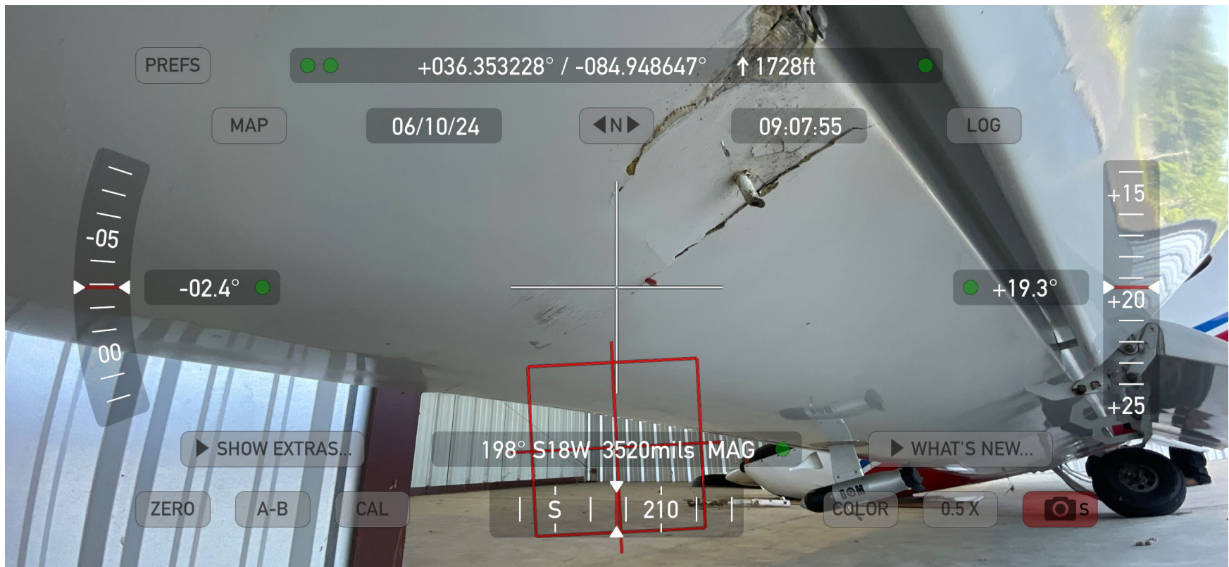
Photograph 3 - FAA Digital Photograph. View of the Bottom of the Left Wing. Note the Chordwise Cracks in the Lower Wing
