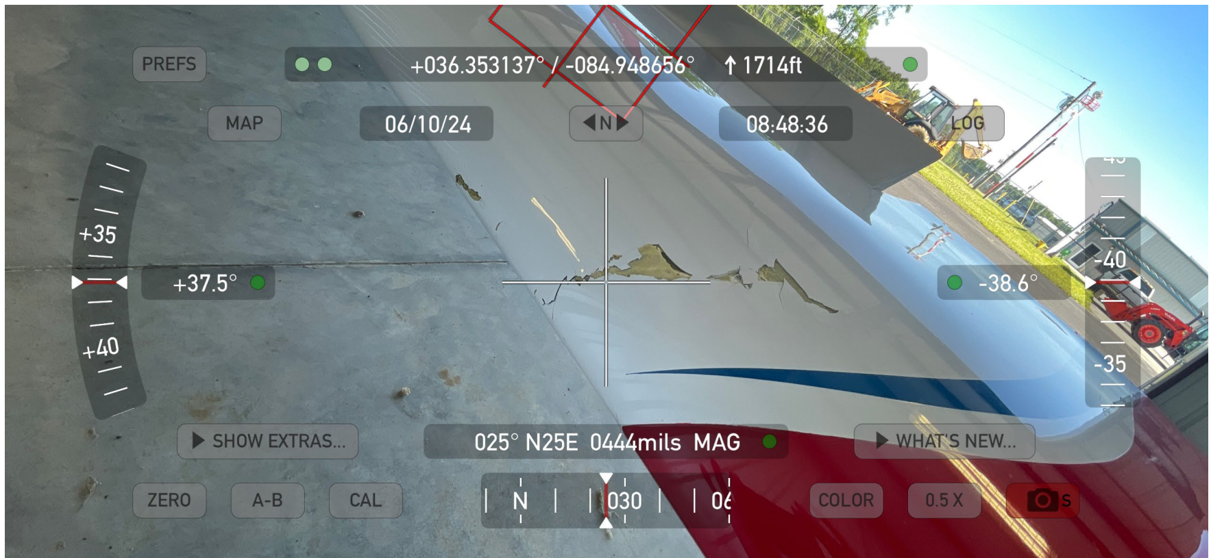
Photograph 4 - FAA Digital Photograph. View of the Outboard Upper Surface of the Left Wing. Note the Cracks
