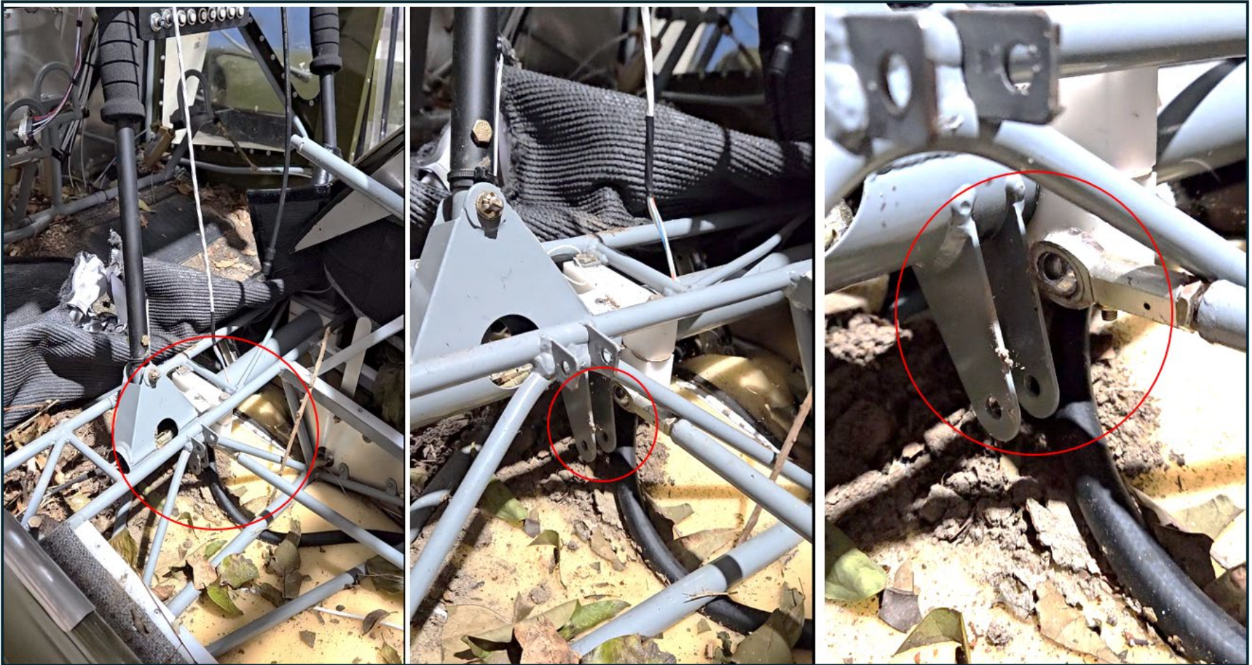
Photo 4: Additional views of the accident airplane missing its elevator connecting rod hardware (screw and locknut) (Photo Courtesy of FAA)
