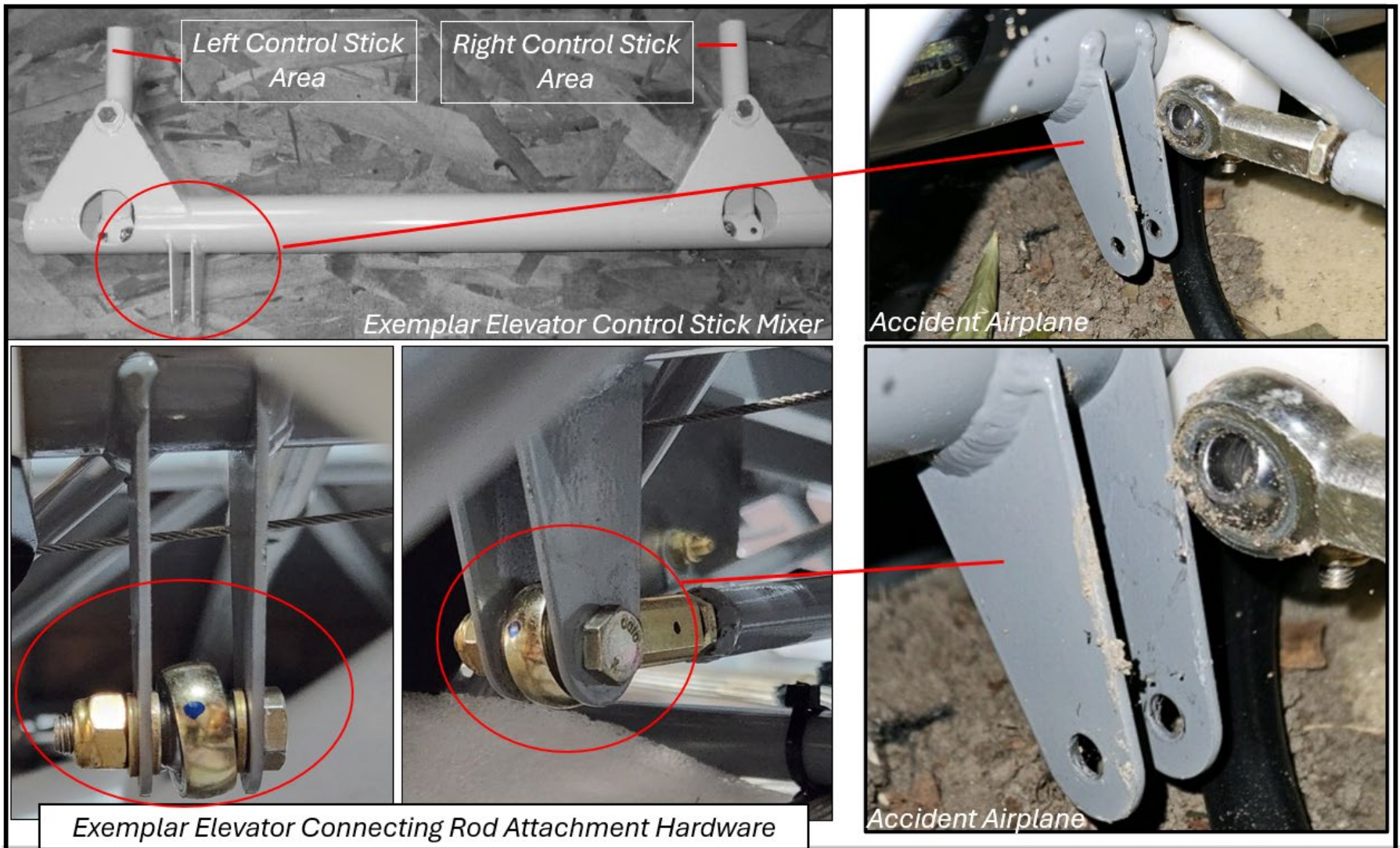
Photo 3: View of the elevator connecting rod attachment areas, exemplar and accident airplane (Photo Courtesy of FAA & Just Aircraft)
