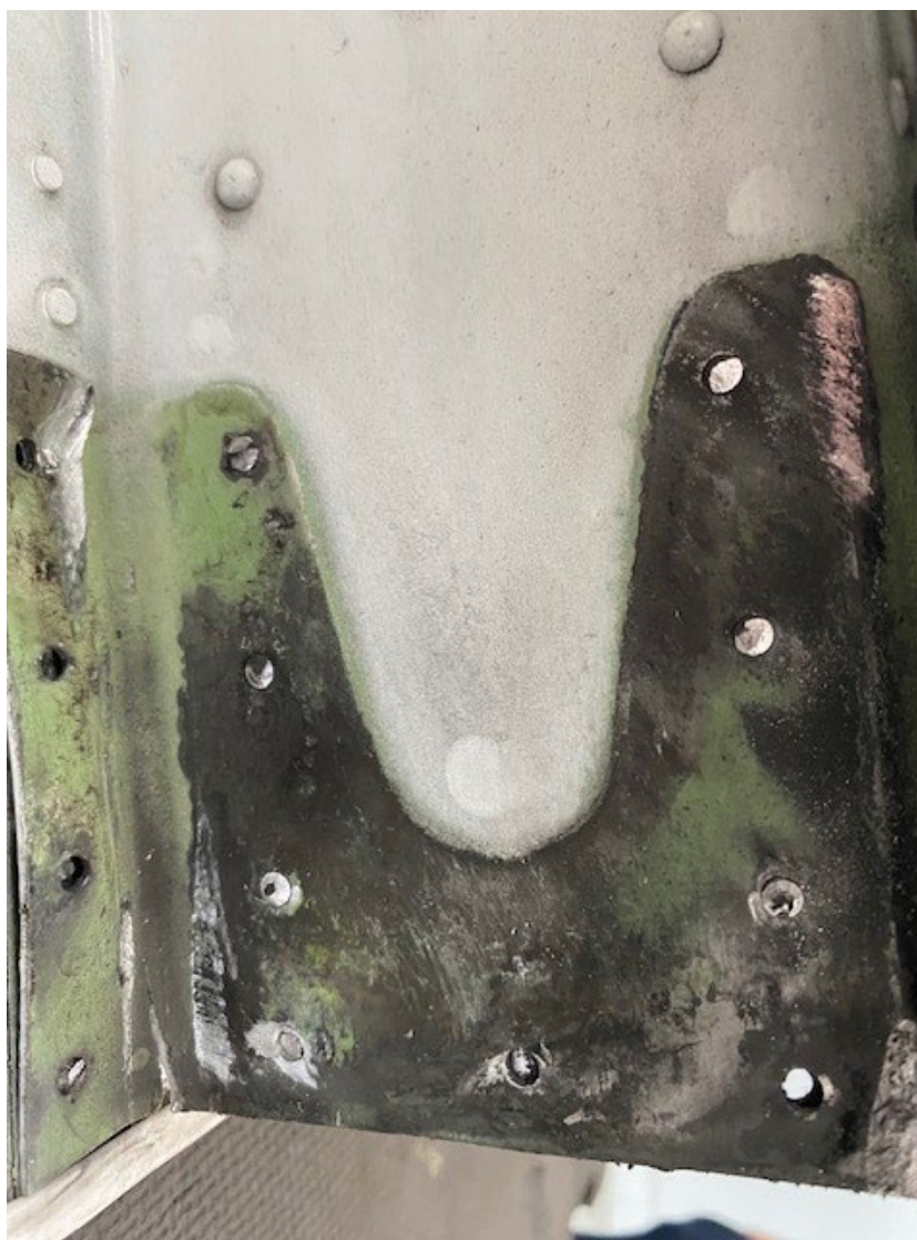
Photograph 4 - Vertical Stabilizer, note: fractured rivets (Courtesy of Skyborne)
