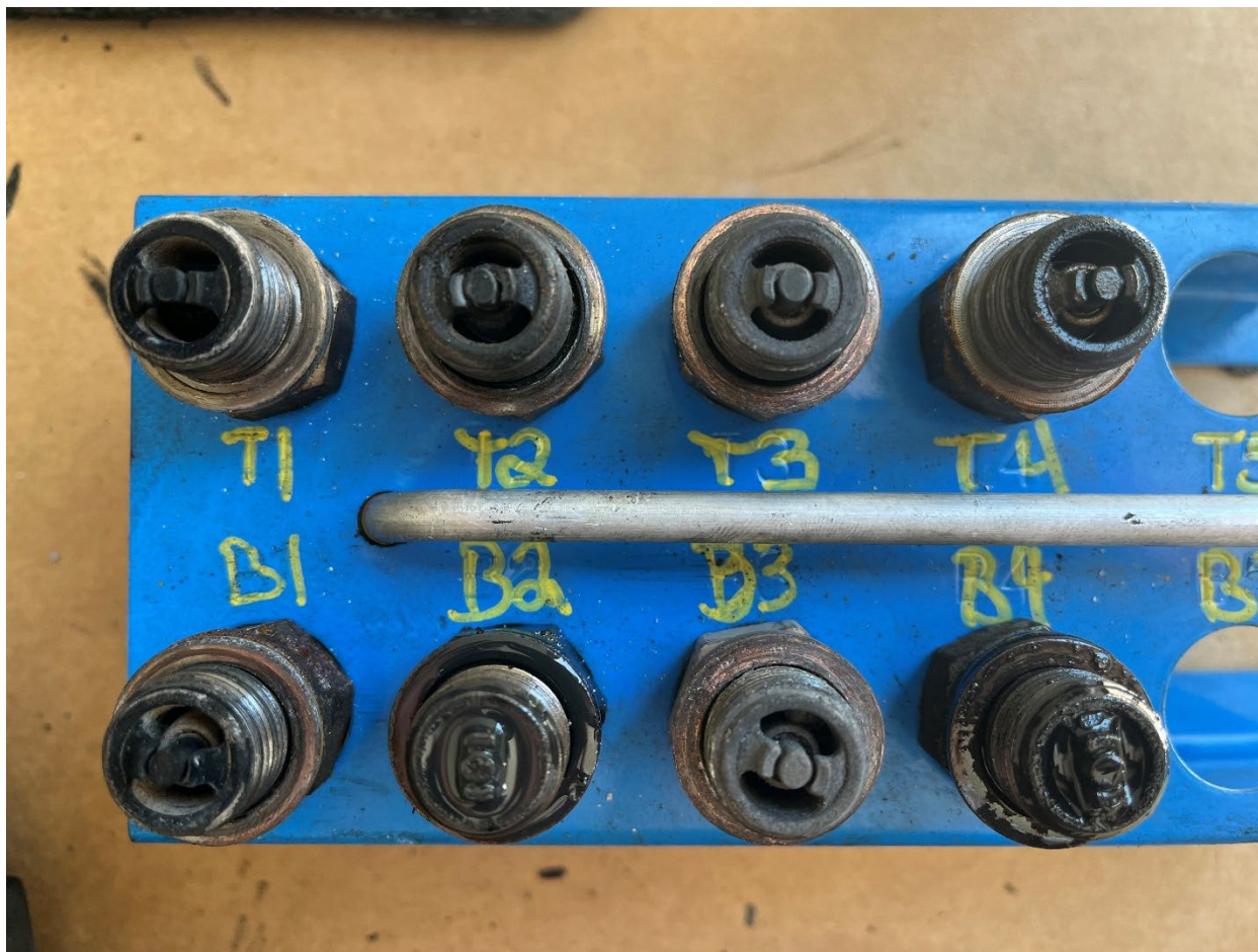
Photograph 10 - View of spark plugs. (Courtesy of Lycoming)
