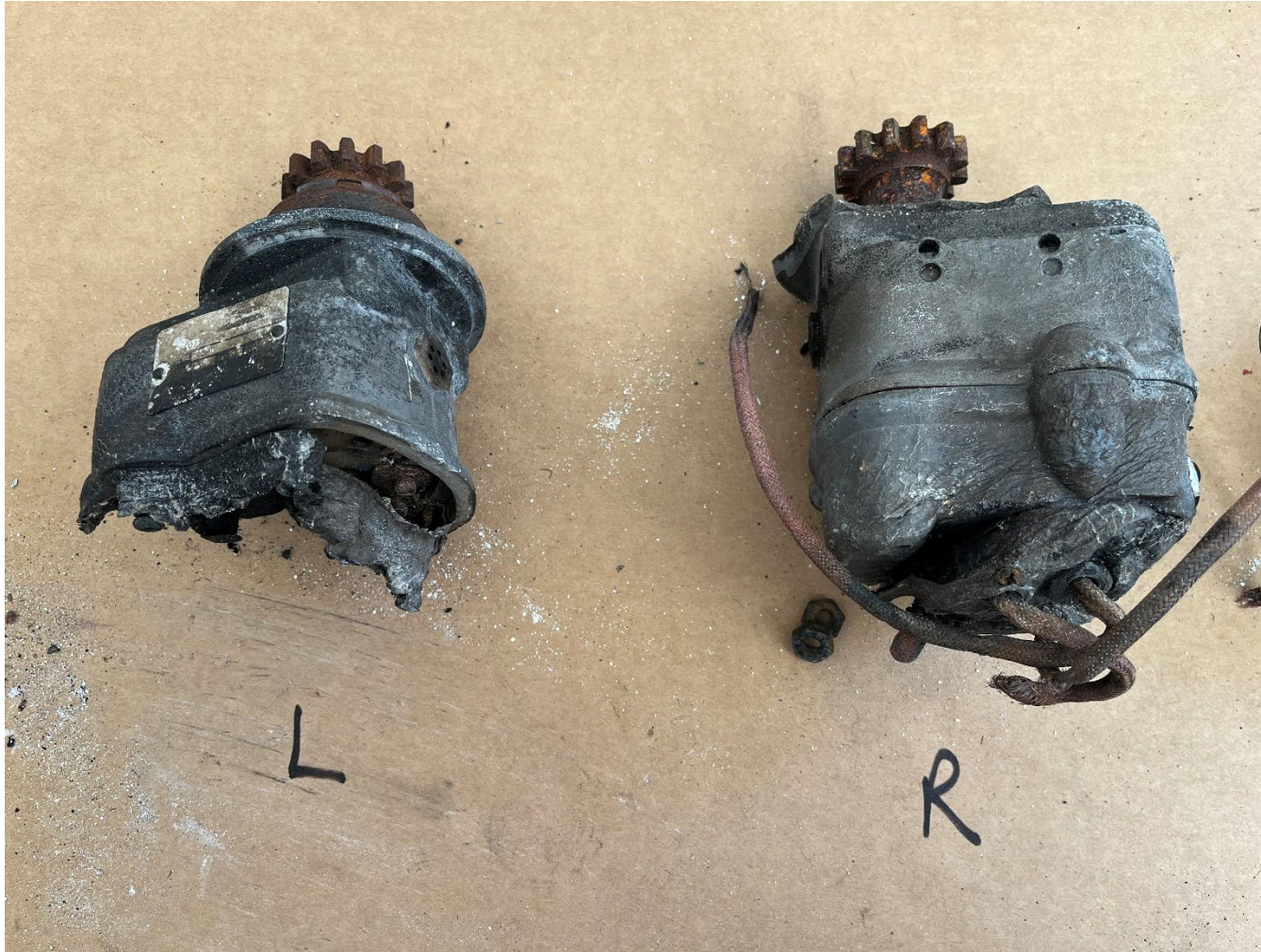
Photograph 9 - View of damaged magnetos. (Courtesy of Lycoming)
