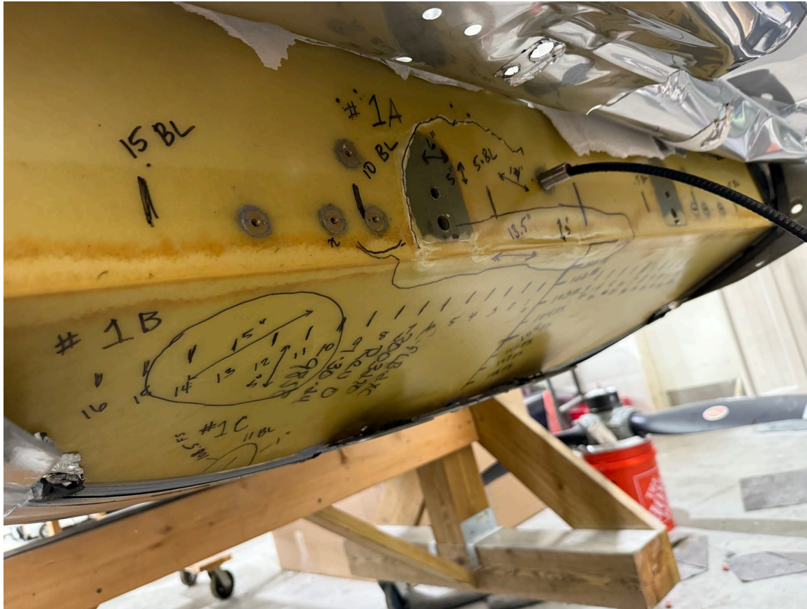
Photograph 3 - Digital Photograph From Repair Facility. View Depicting Cracks in the Structural Firewall
