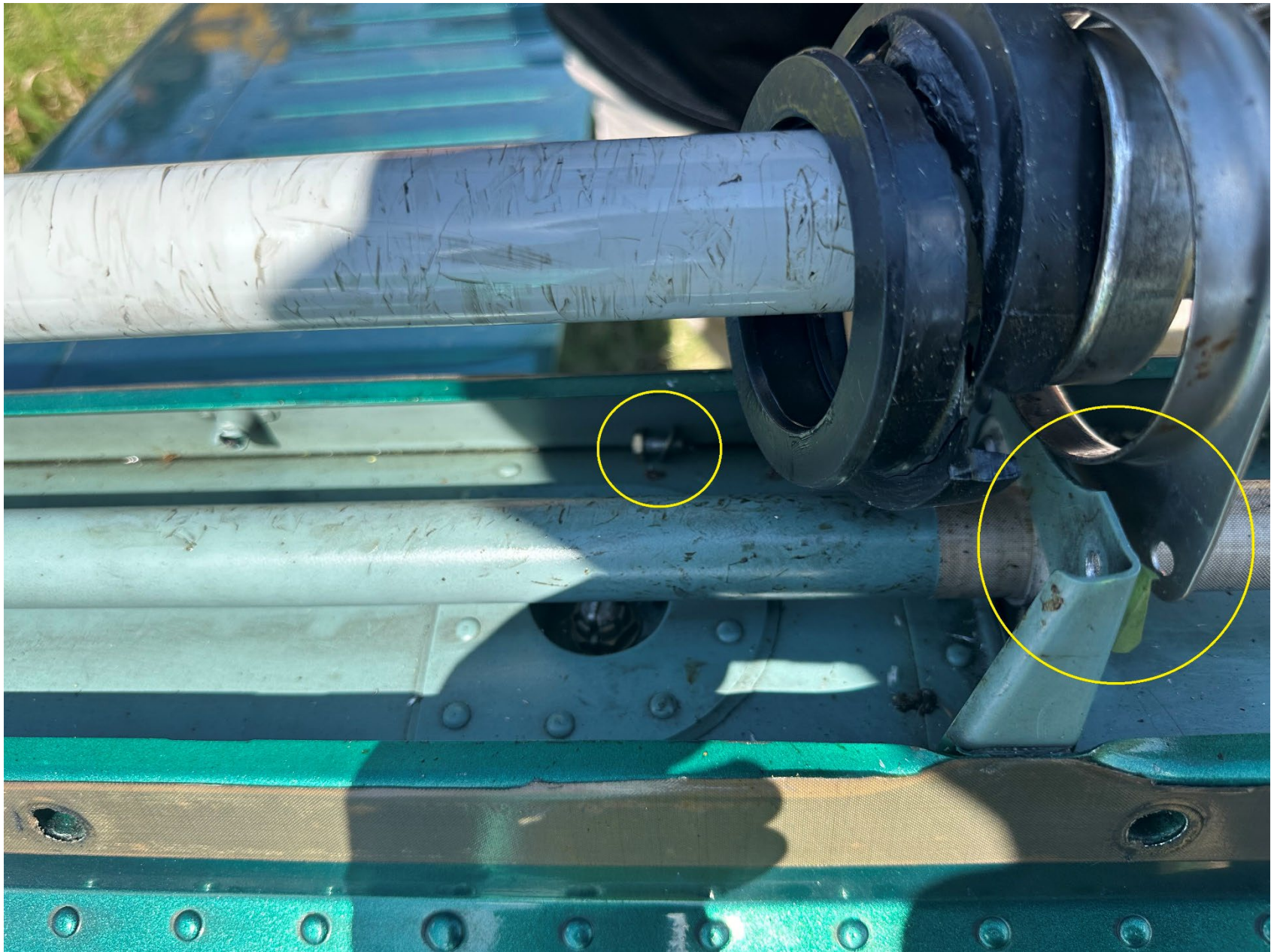
Photo 3 – View of Dismounted and Damaged No. 1 T/R Driveshaft Bearing (HCSO)
