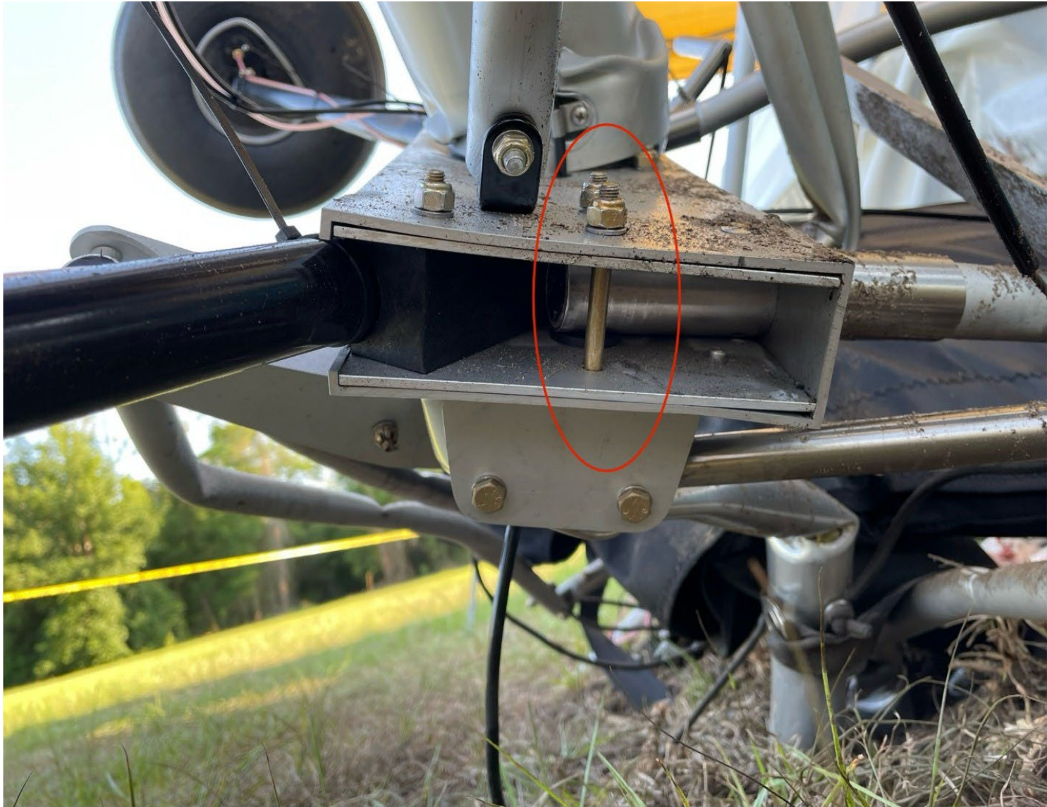
Photograph 5 - Fuselage connection point with bolt shown installed. (Courtesy of FAA)
