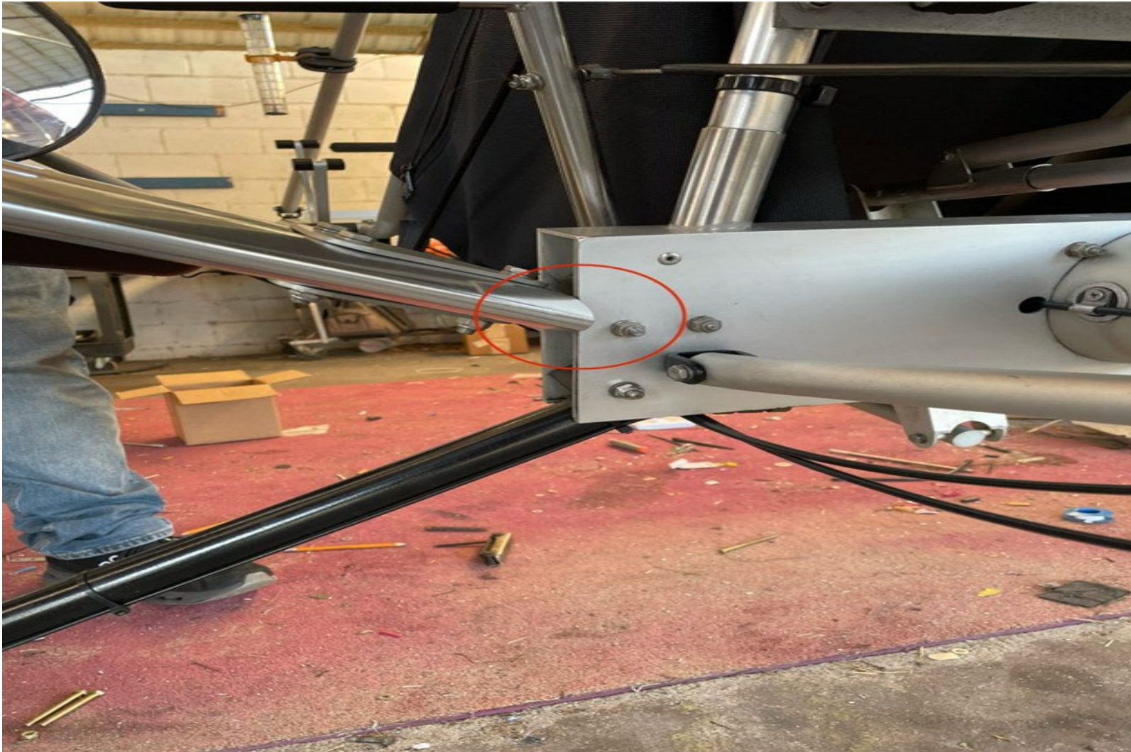
Photograph 6 - Wing connection point properly installed - Non-Accident Aircraft Side 1 (Courtesy of FAA)
