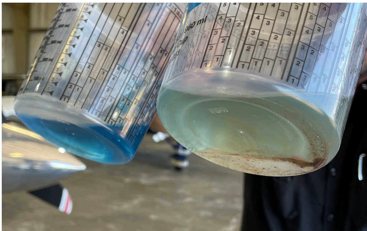
Photograph 7 - Fuel from left wing (left) and from gascolator and carburetor bowls (right).
