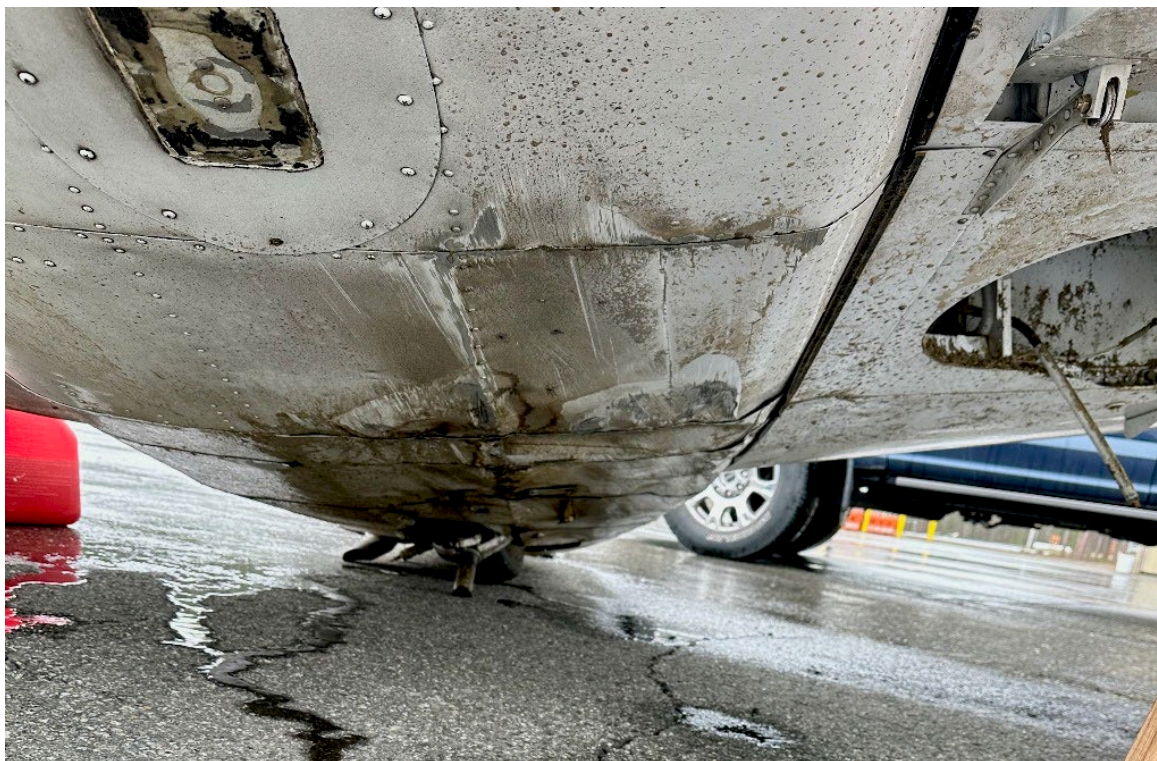
Photograph 4 - Damage to lower fuselage (Courtesy of Murray Collette, pilot/owner)
