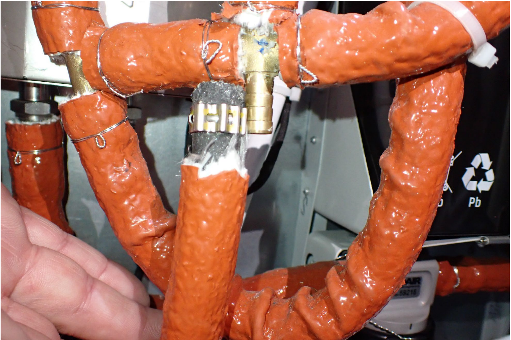
Photograph 6 – Disconnected fuel line lined up with the four-way distributor
