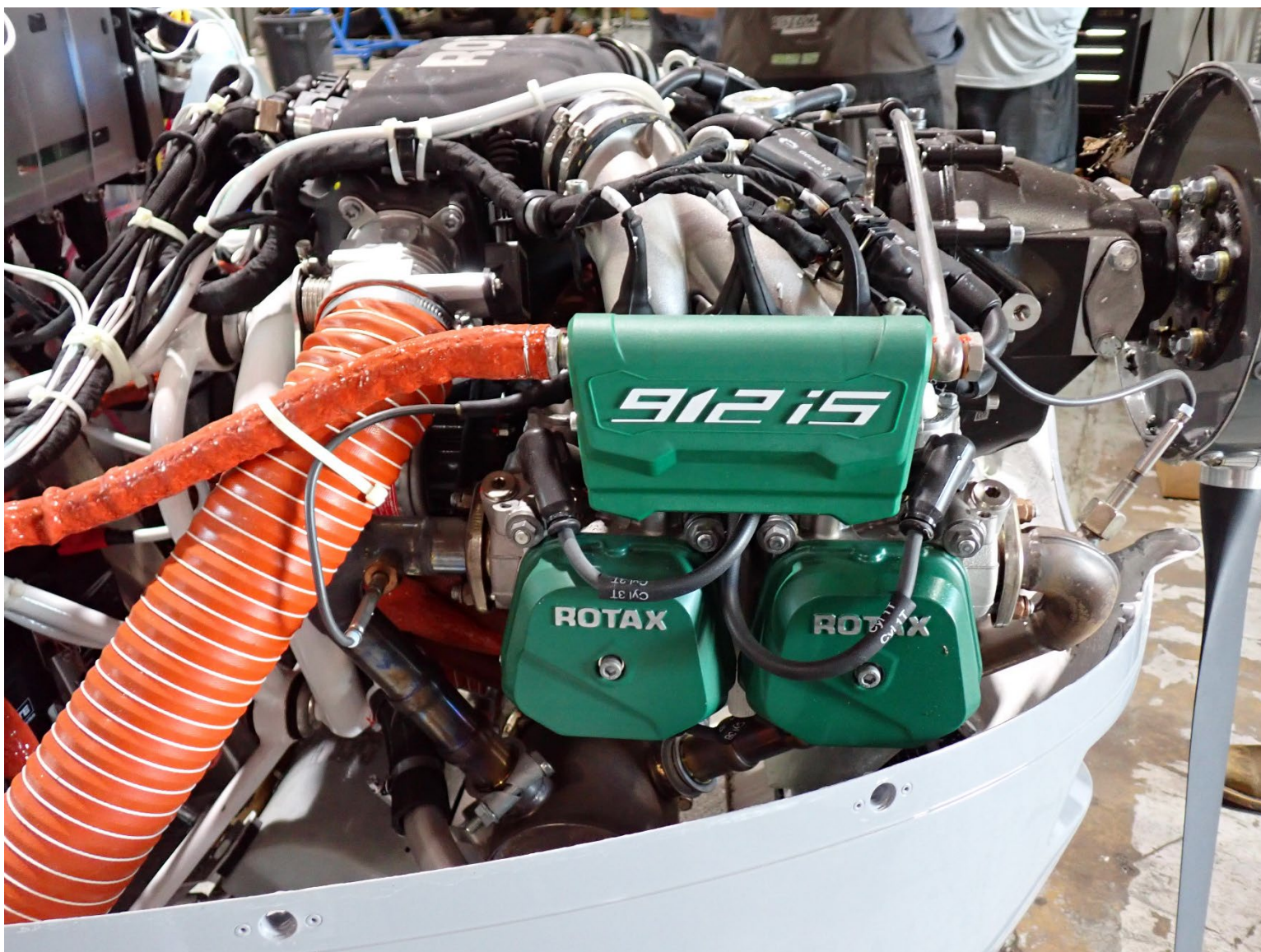
Photograph 8 – Engine overview
