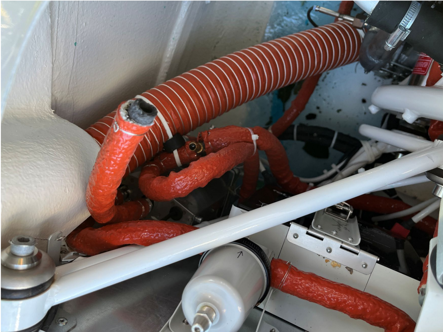
Photograph 3 – Disconnected fuel line found at the accident site (Courtesy of FAA)
