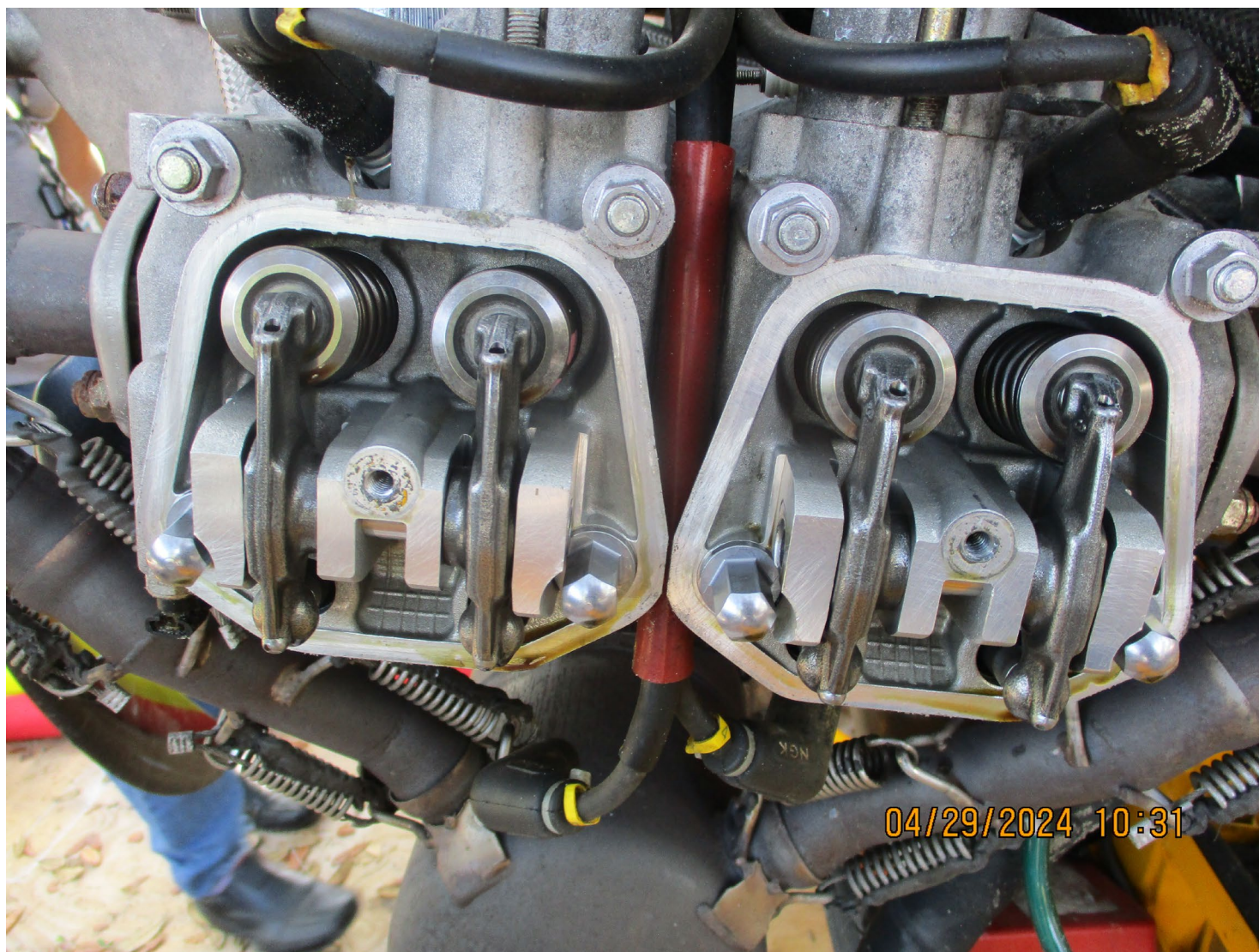
Photograph 3 - Rocker Arms and springs, (Note: lack of oil)
