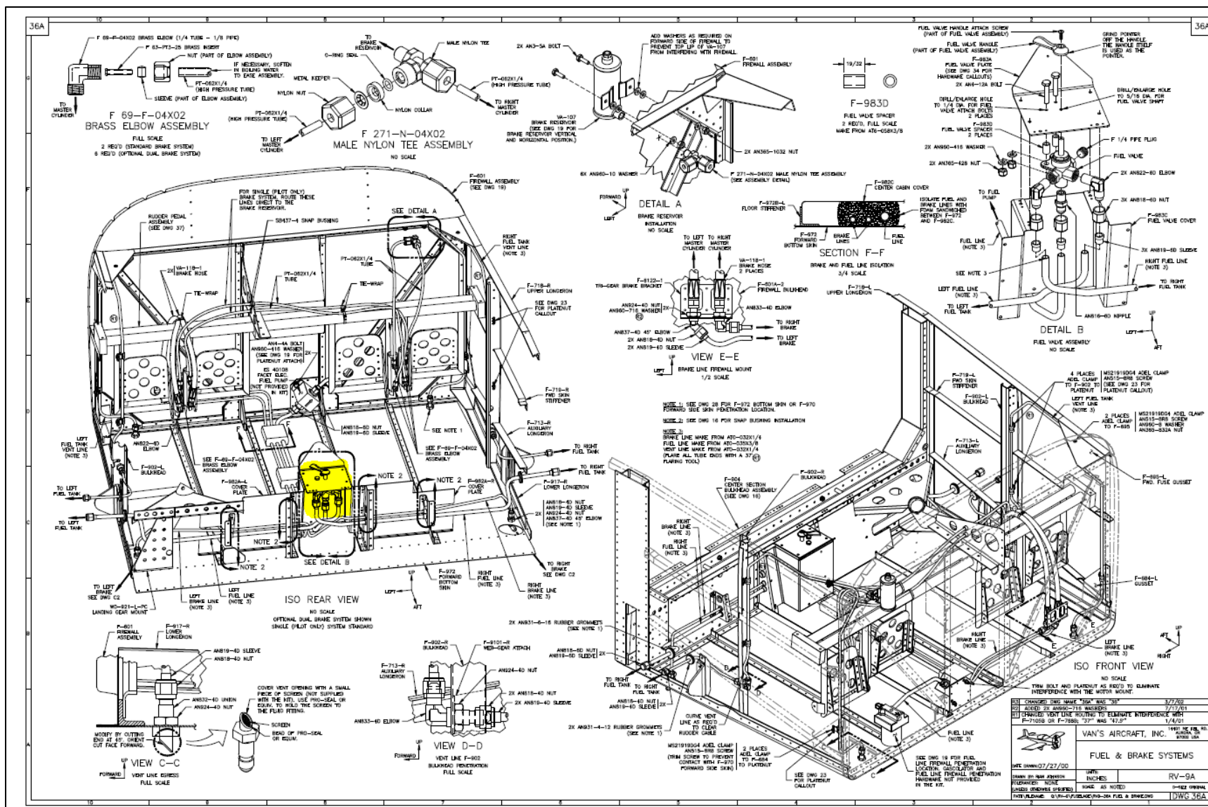
Photo 4: View of the airplane build drawing with the fuel selector highlighted.
