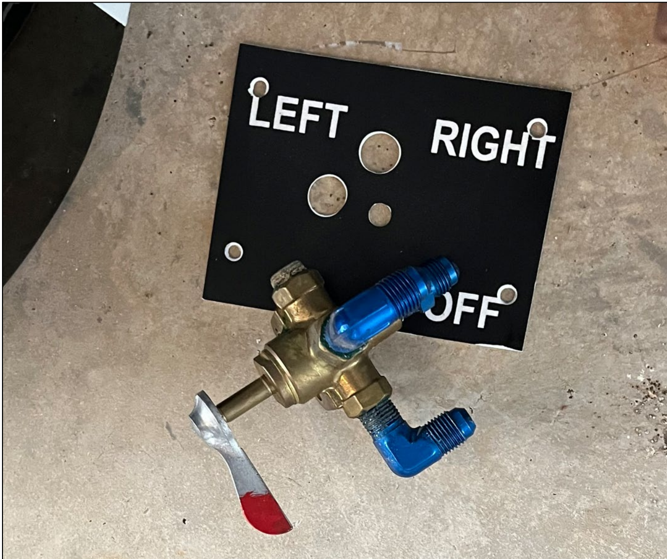
Photo 3: View of the fuel selector removed from the airplane during examination (Photo Courtesy of FAA)
