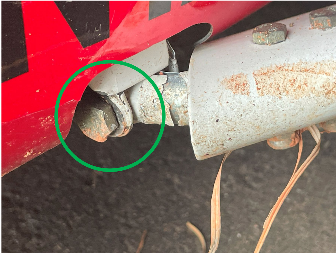
Photograph 3 - Bent Structure at Main Landing Gear (Courtesy of Owner)
