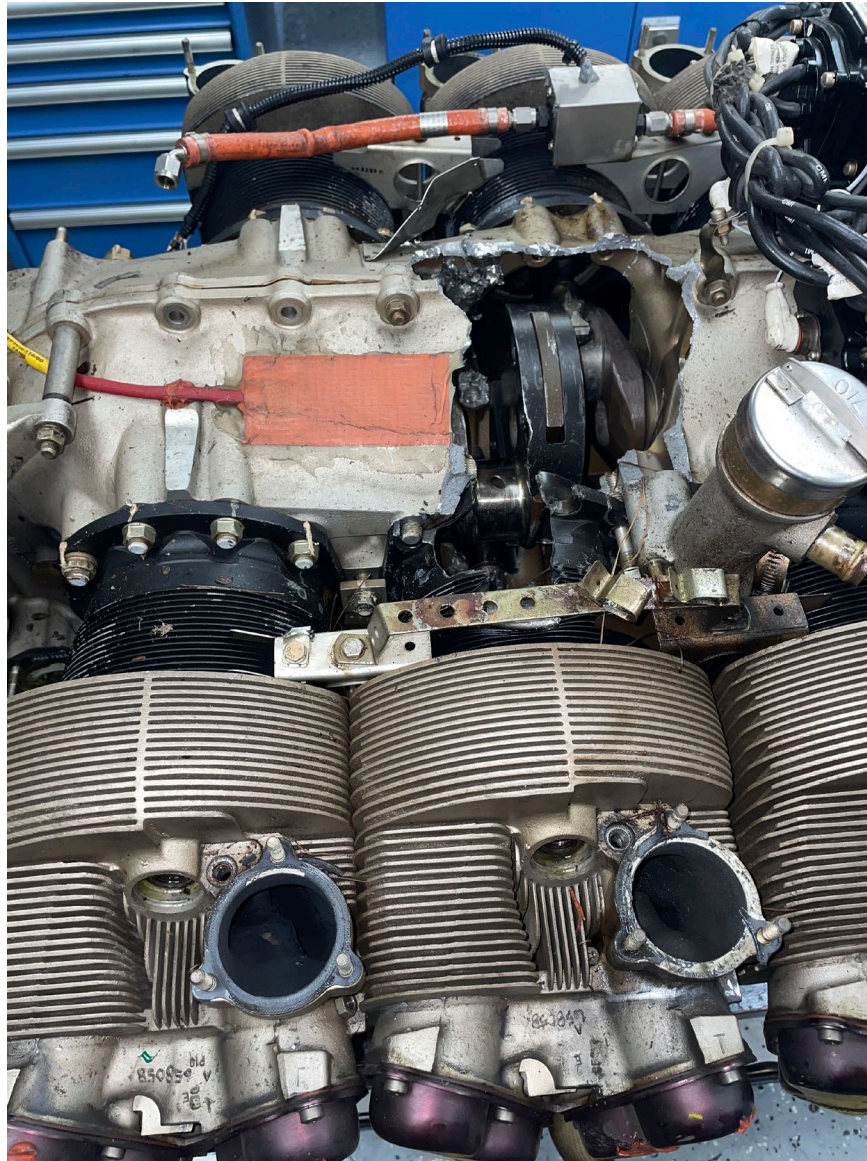
Photograph 3 - Hole in top of engine. (NTSB)
