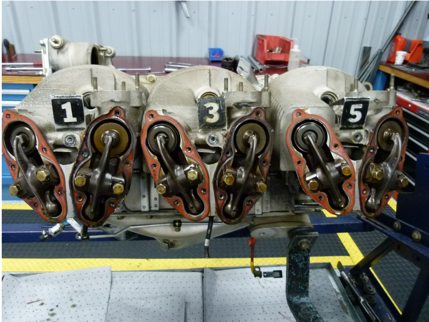
Photograph 6 - Engine, number 1,3,5 side. (NTSB)
