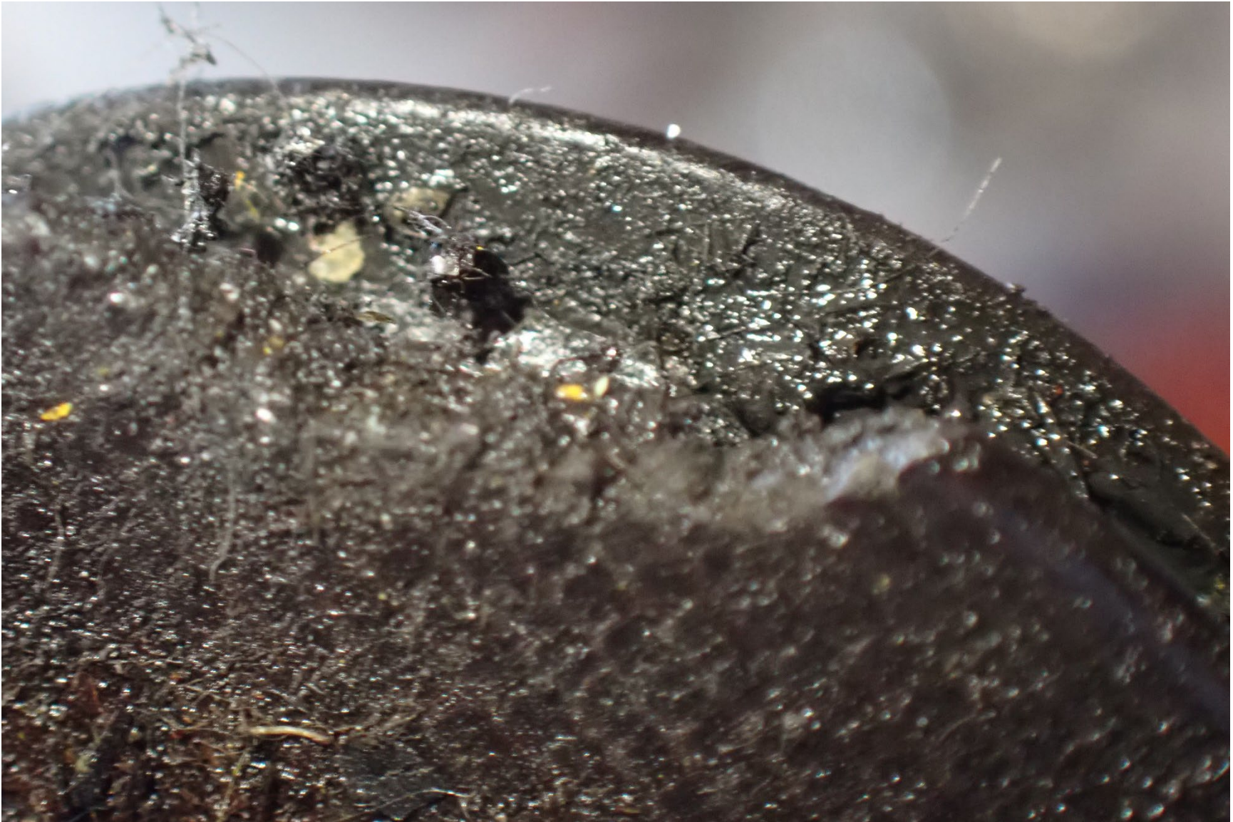
Photograph 13 - Close up view of the lower left fuselage aileron pulley
