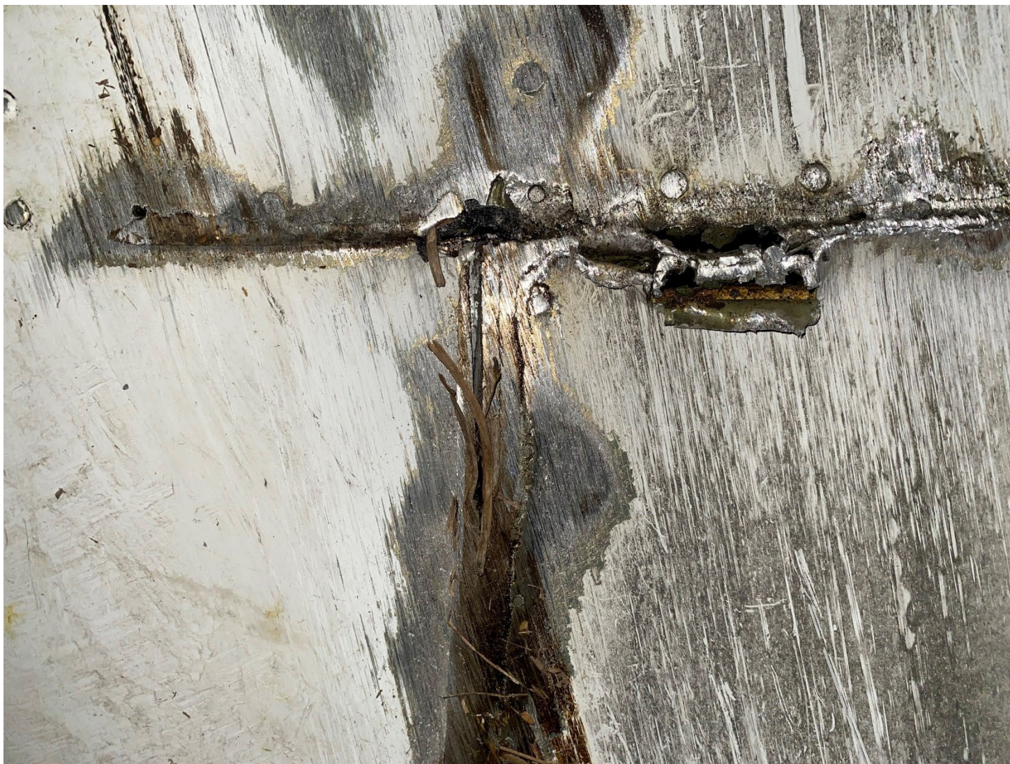
Photograph 3 - Close-up view of fuselage damage. (Courtesy of pilot)
