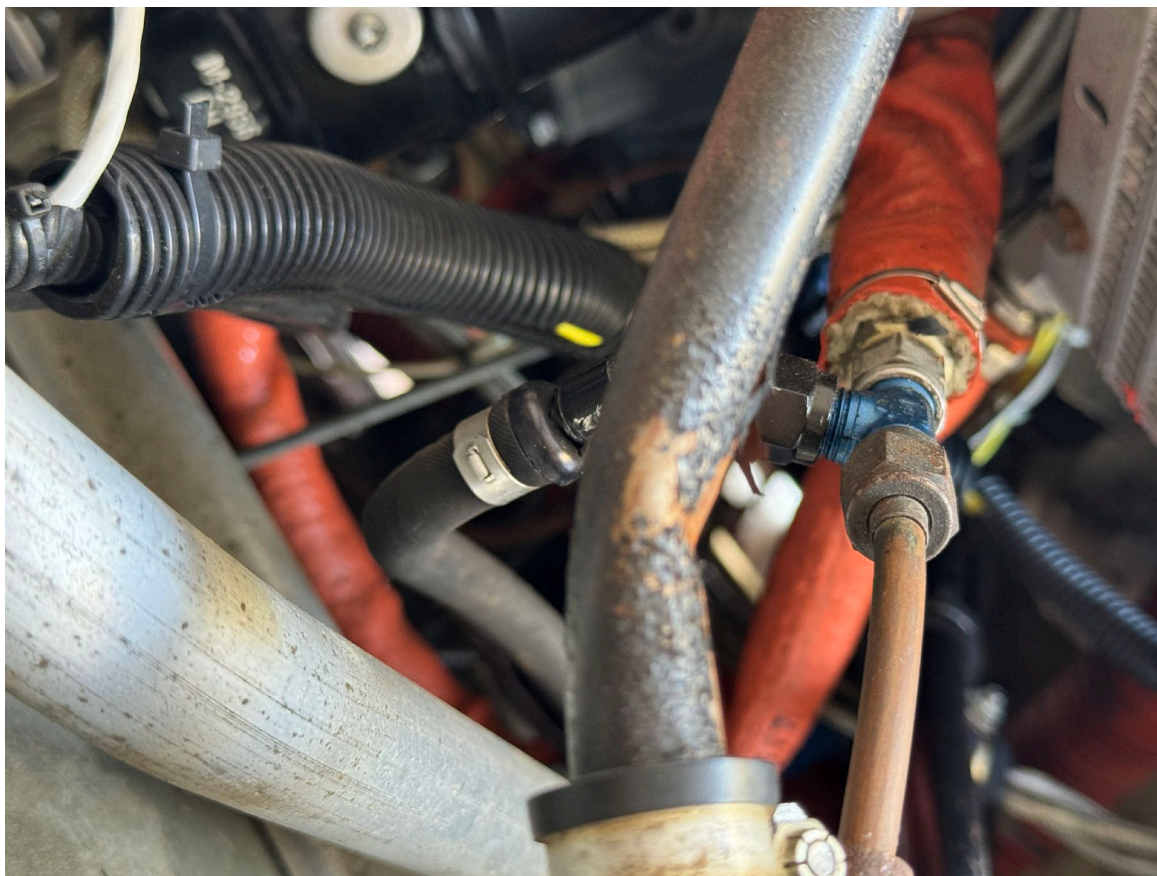
Photograph 2 - View of damage to the engine mount. (Courtesy of FAA)
