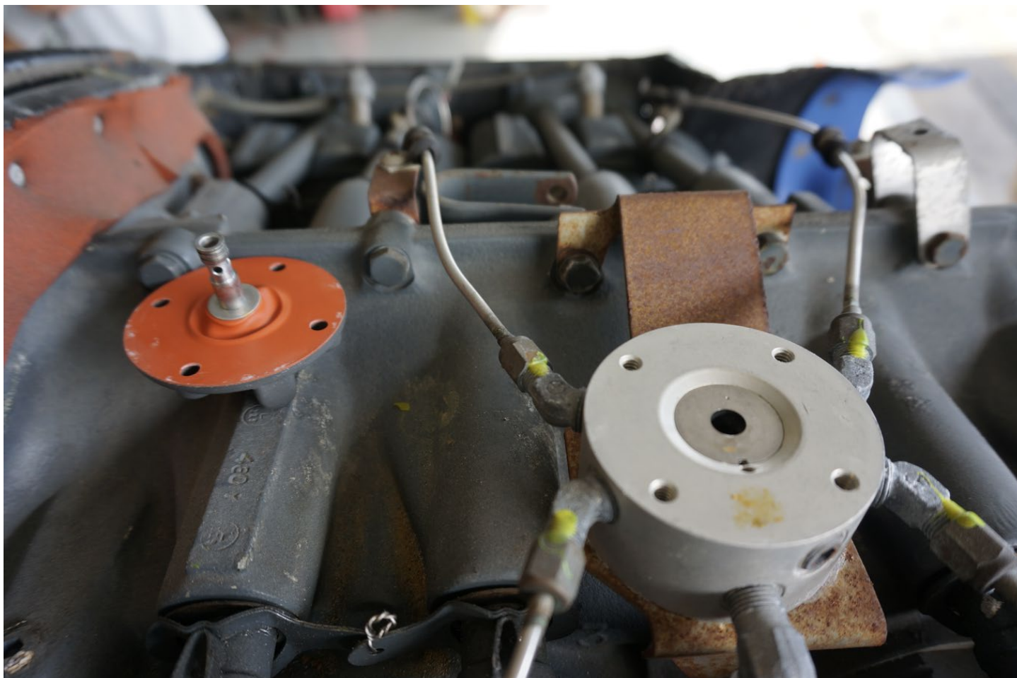
Photograph 20 - Fuel Distribution Manifold
