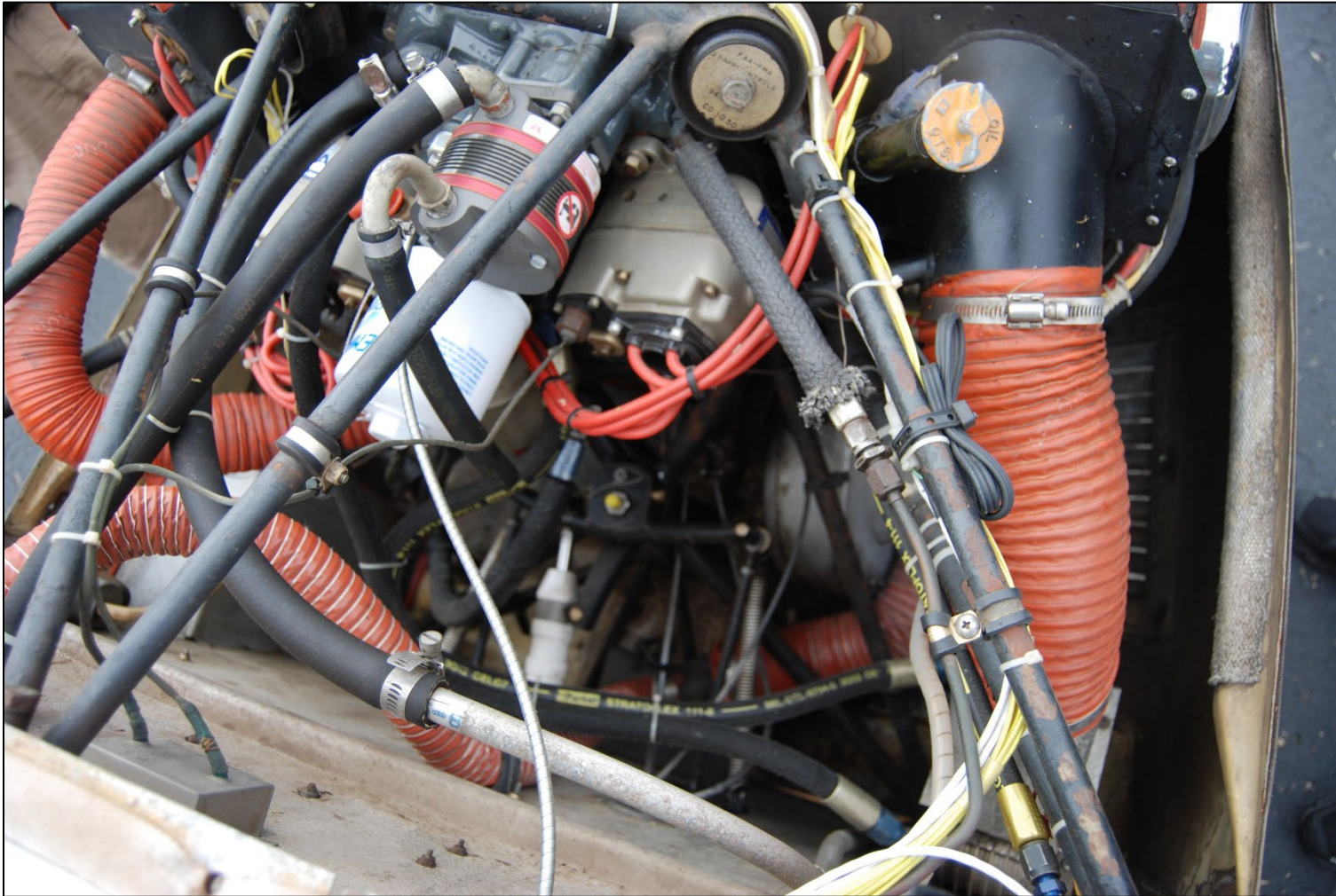
Figure 3: View of the engine compartment. Note the engine mount was substantially damaged. (Photo Courtesy of FAA)
